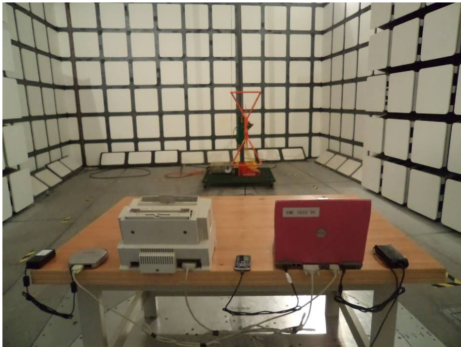
Spurious Radiated Emissions - Rear View (Downloading mode)
