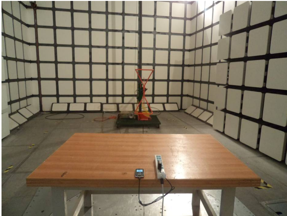
Radiated Emissions - Rear View (Charging & Media Playing)
