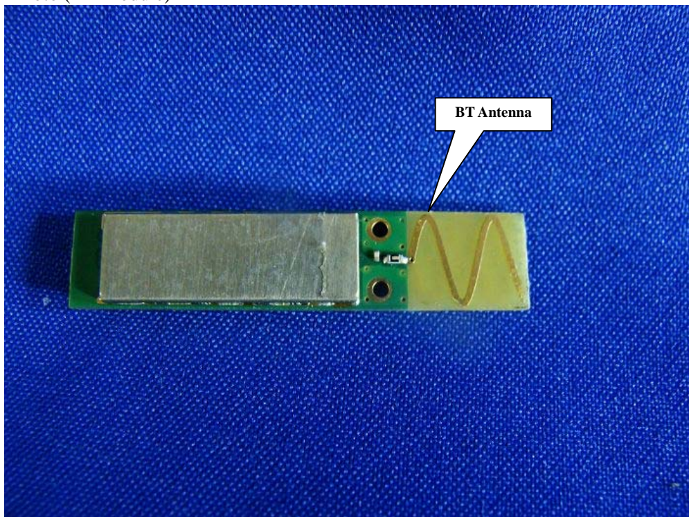
(14) EUT Photo (BT Module)
