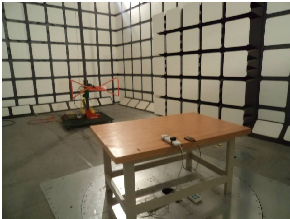
Radiated Emissions - Rear View (charging & playing mode)
