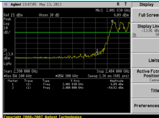
Hopping mode
