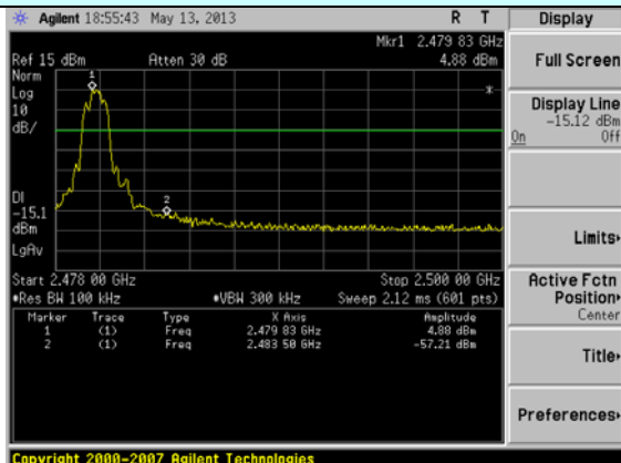
No-hopping mode
