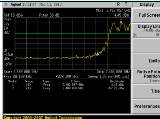
Hopping mode
