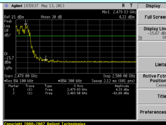
Hopping mode
