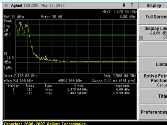
Hopping mode
