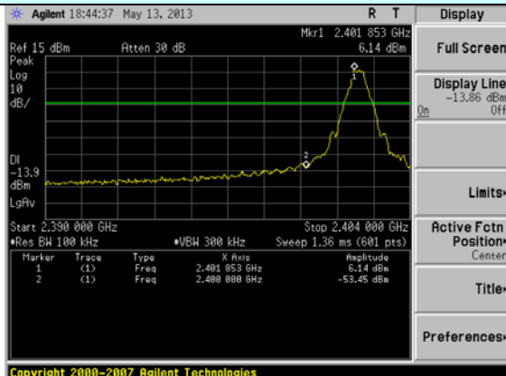
No-hopping mode
