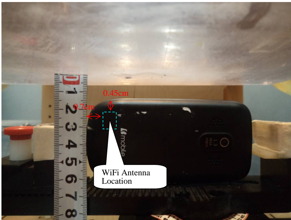
WiFi Body-Right Setup Photo
