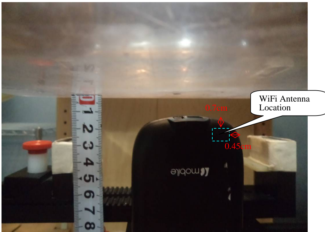
WiFi Body-Bottom Setup Photo
