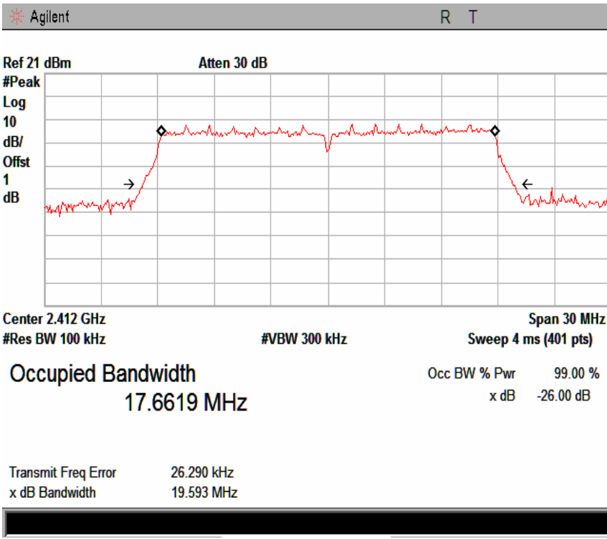
802.11n-26dB-low
