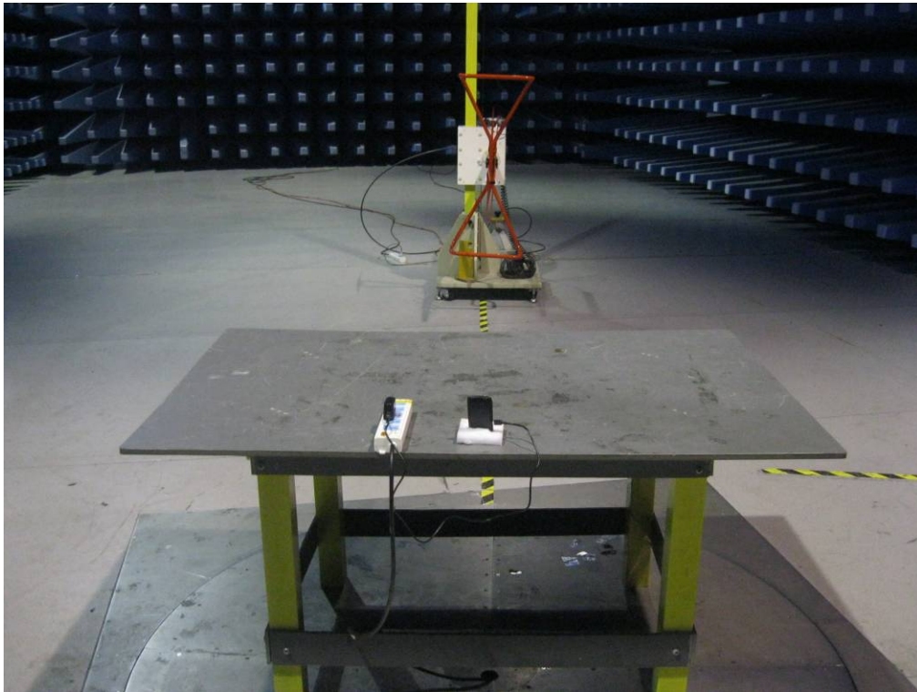
Radiated Emissions Test Setup Below 1GHz (GPS receiving) - Front View
