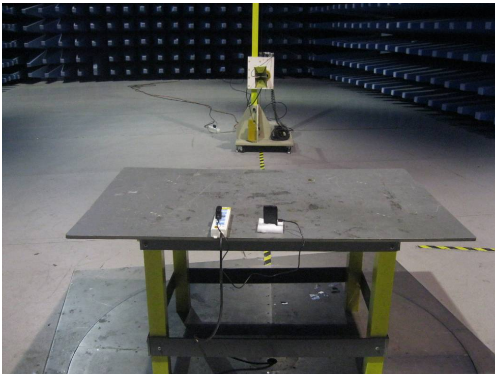
Radiated Emissions Test Setup Above 1GHz (GPS receiving) - Front View
