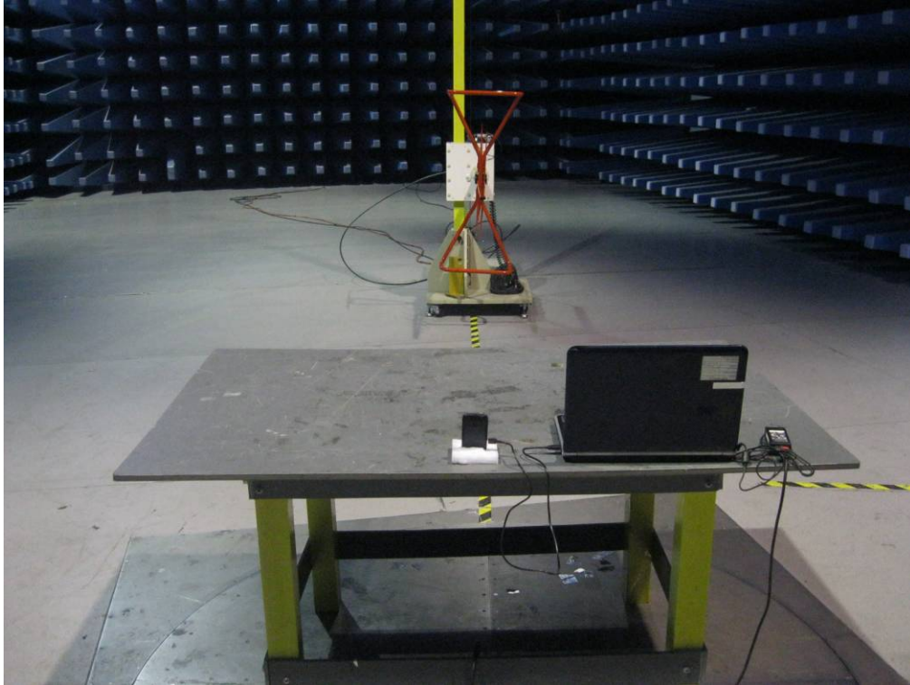
Radiated Emissions Test Setup Below 1GHz (Charging& Downloading) - Rear View
