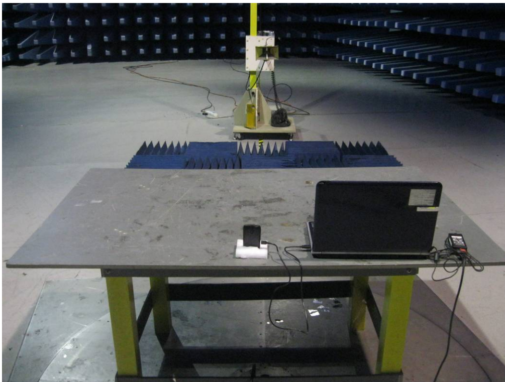
Radiated Emissions Test Setup Above 1GHz (Charging& Downloading) - Rear View
