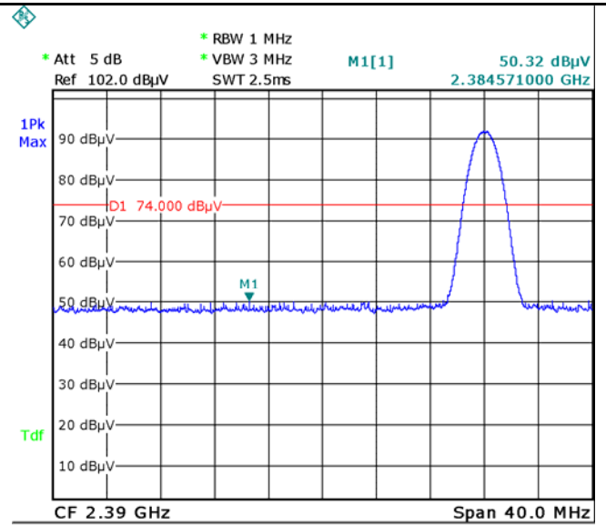
8DPSK-Left Side-PK
