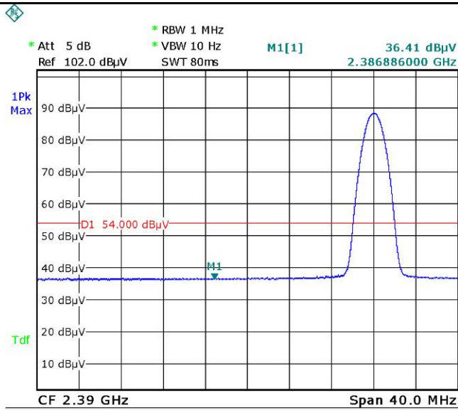
8DPSK-Left Side-Ave
