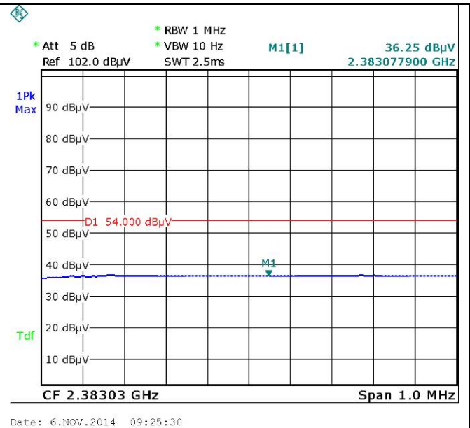
8DPSK-Hopping-Ave-Left Side
