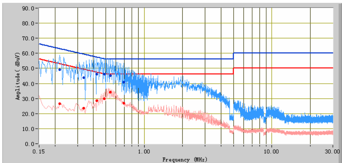
Phase Neutral Plot at 120Vac, 60Hz
