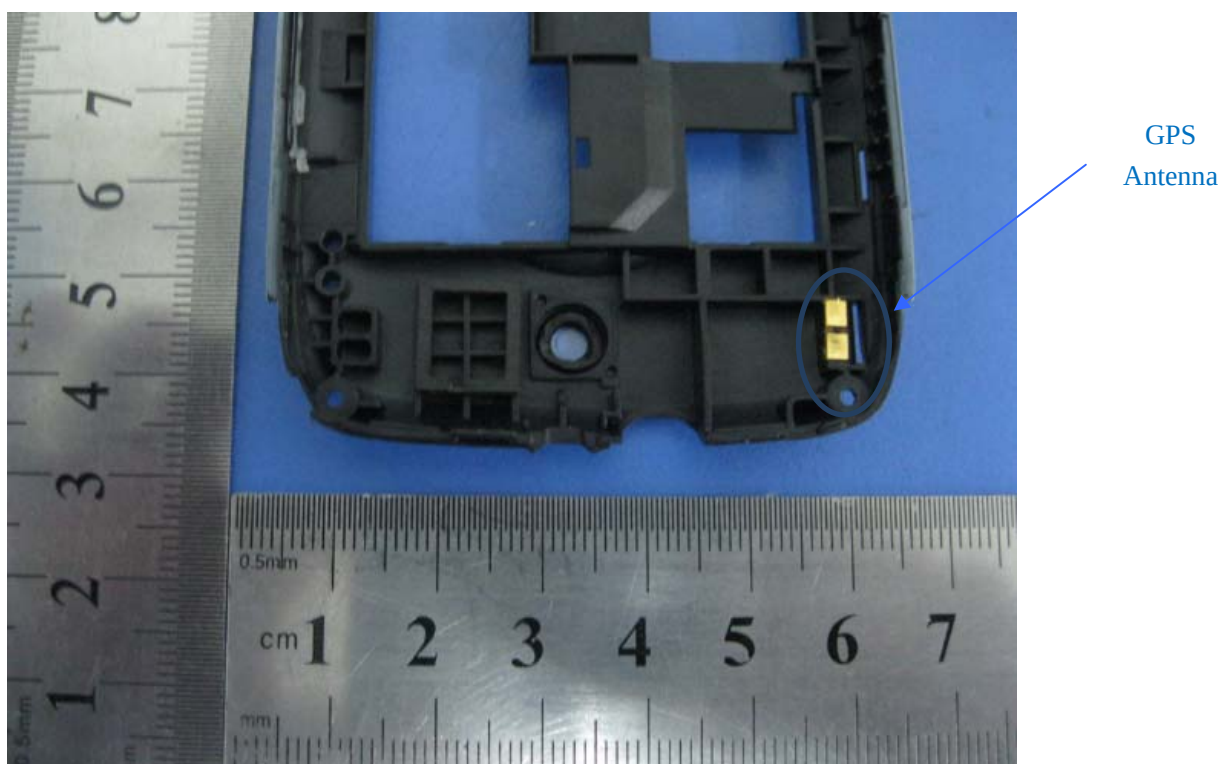
GPS Antenna - Top View
