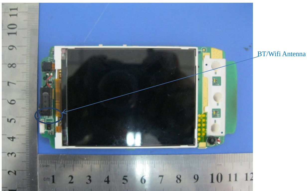
BT/Wifi Antenna - Top View
