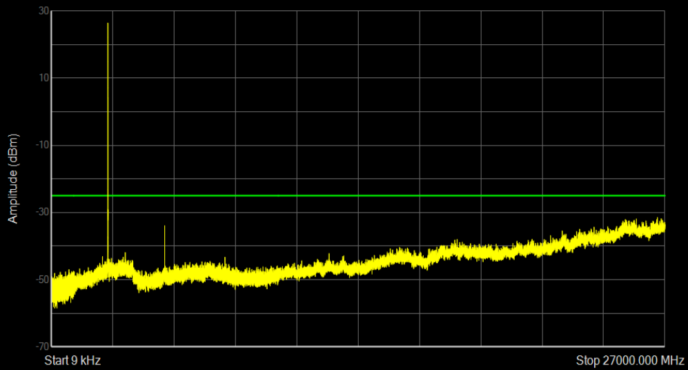
Band7 16QAM BW=5MHz Channel=20775 RB Size=1 Position=#0
