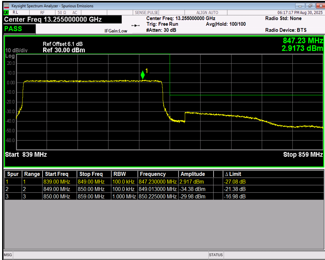
Band5 64QAM BW=10MHz Channel=20600 RB Size=1 Position=#0
