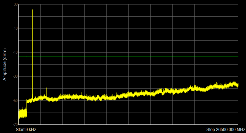
Band66 QPSK BW=1.4MHz Channel=131979 RB Size=1 Position=#0
