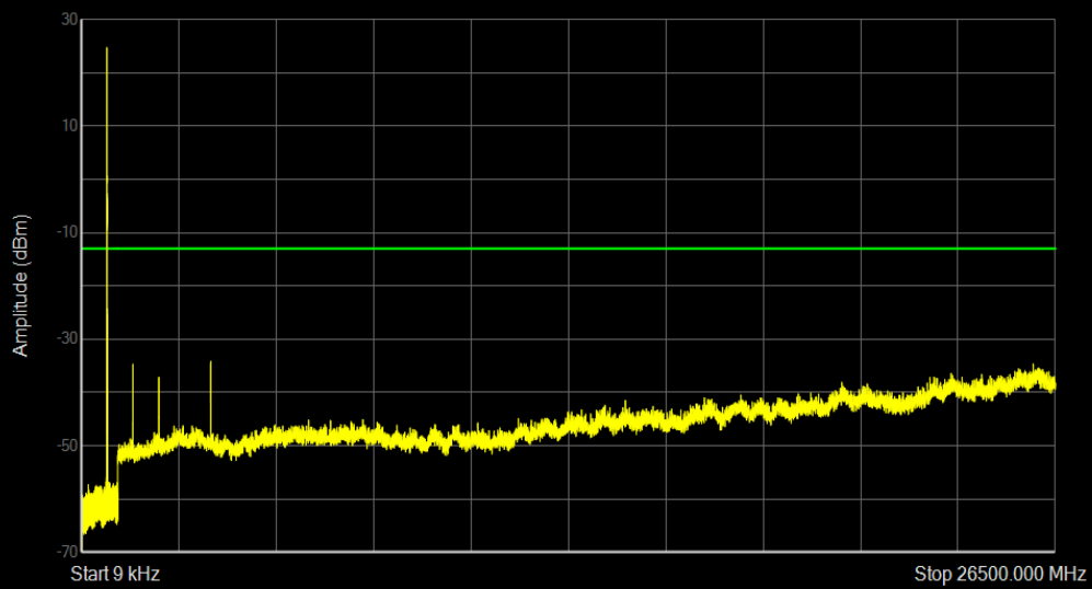
Band12 16QAM BW=3MHz Channel=23095 RB Size=1 Position=#0
