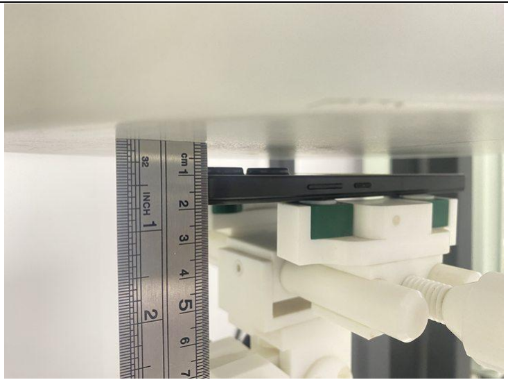
Right Side (Separation distance of 10mm)
