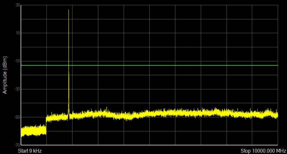
Band2 QAM16 BW=5MHz Channel=18900 RB Size=1 Position=#0
