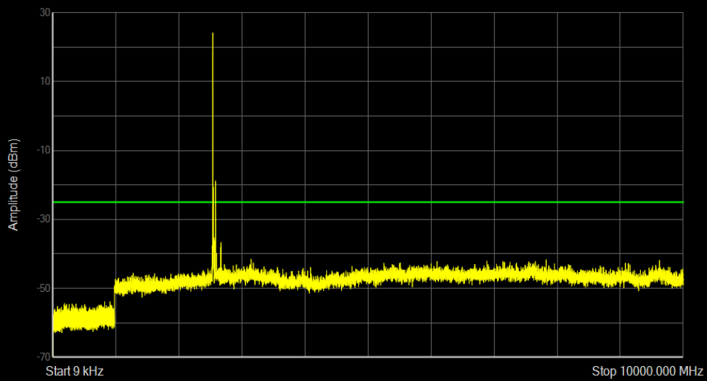
Band41 QPSK BW=20MHz Channel=40340 RB Size=1 Position=#0
