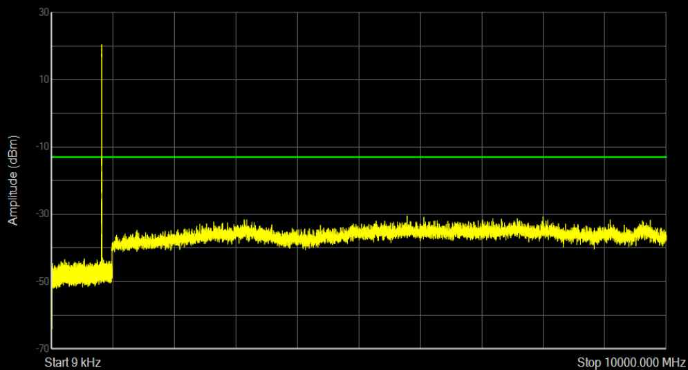
Band5 QAM16 BW=1.4MHz Channel=20525 RB Size=6 Position=#0
