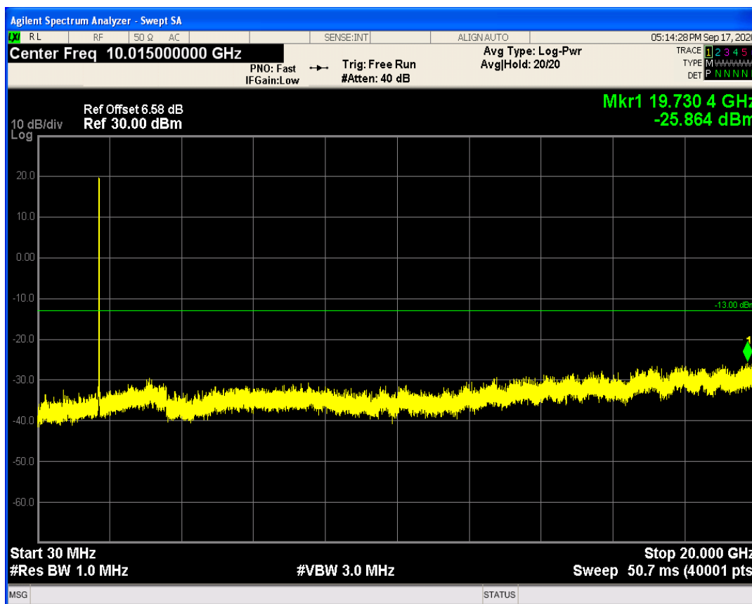
LTE Band4 QPSK BW=10MHz Channel=20350 RB Size=1 Position=#0
