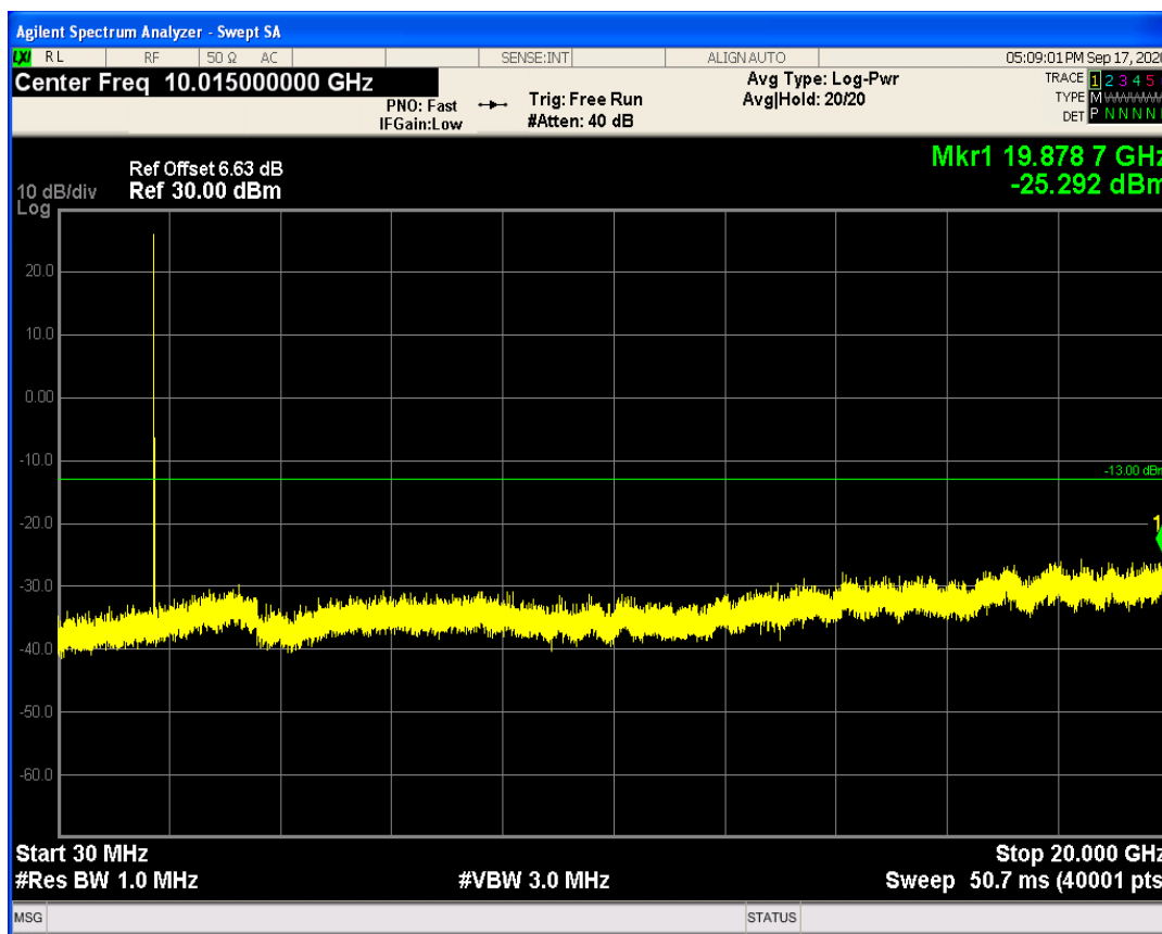
LTE Band4 QPSK BW=5MHz Channel=20375 RB Size=25 Position=#0
