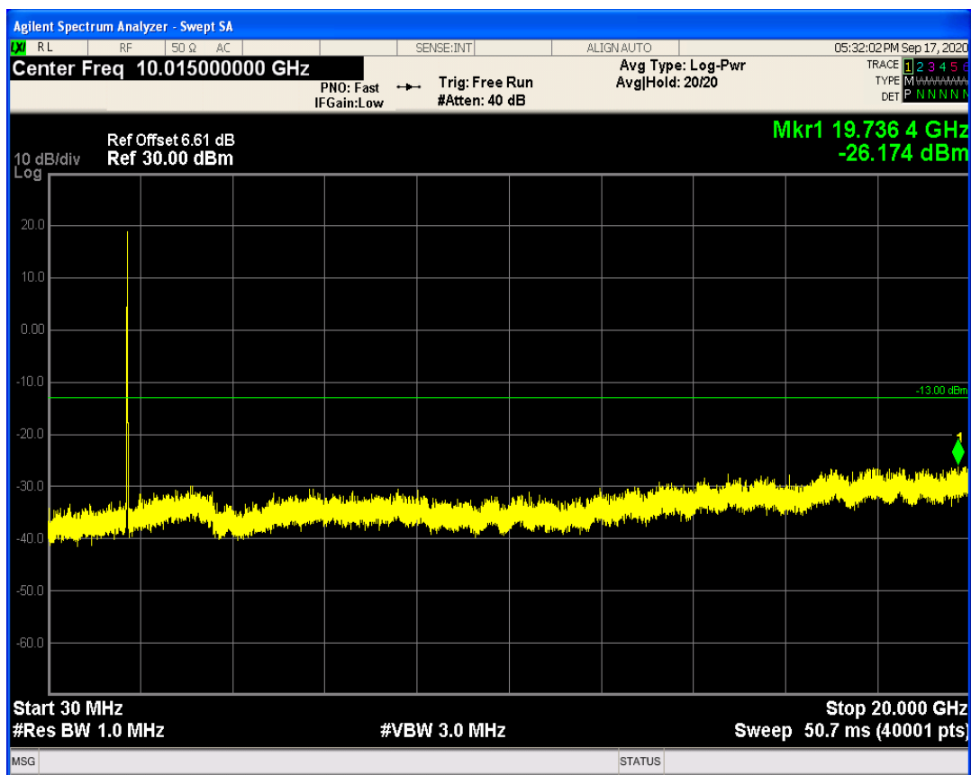
LTE Band5 QPSK BW=1.4MHz Channel=20407 RB Size=1 Position=#0
