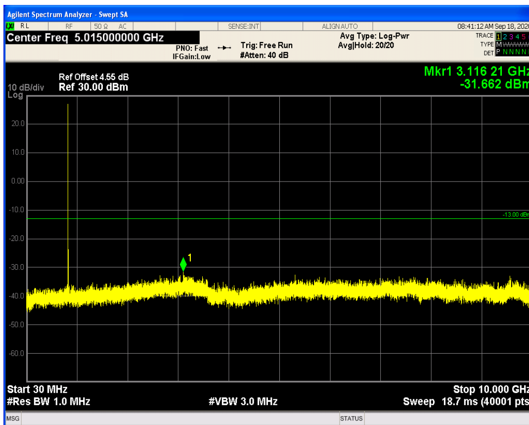
LTE Band5 QPSK BW=3MHz Channel=20635 RB Size=15 Position=#0
