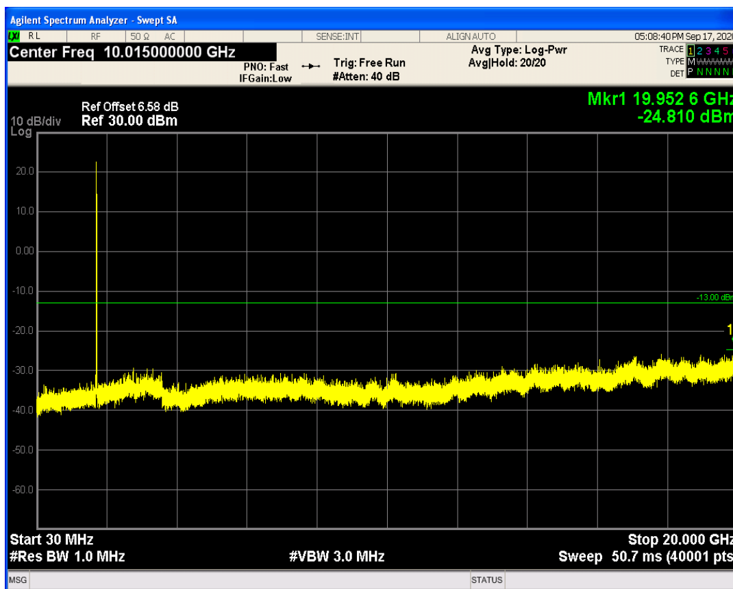
LTE Band4 QPSK BW=5MHz Channel=20375 RB Size=1 Position=#0
