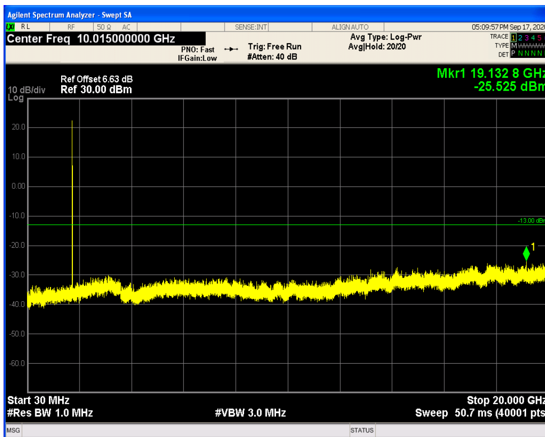
LTE Band4 QPSK BW=10MHz Channel=20000 RB Size=1 Position=#0
