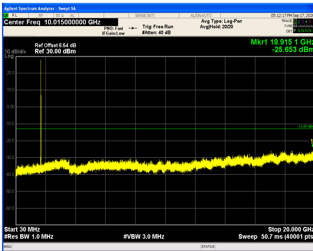
LTE Band4 QPSK BW=10MHz Channel=20000 RB Size=50 Position=#0
