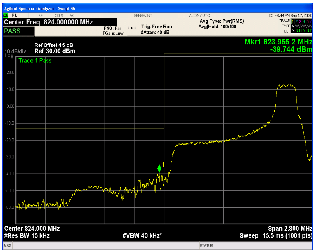
LTE Band5 QPSK BW=1.4MHz Channel=20407 RB Size=6 Position=#0
