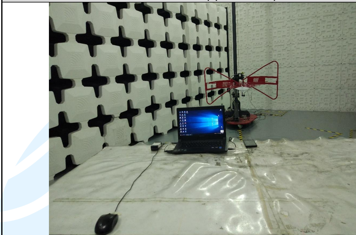
Radiated emission Test Setup (30 MHz~1 GHz) - Mode 6
