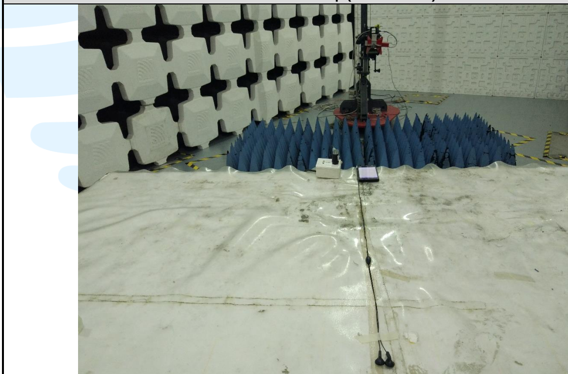
Radiated emission Test Setup (Above 1 GHz) - Mode 1
