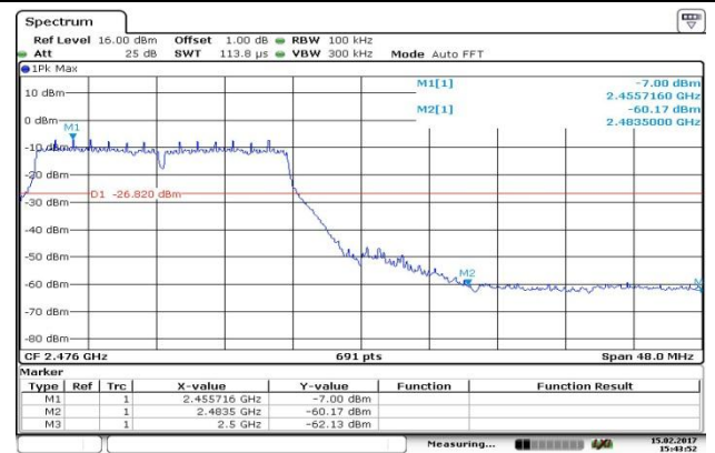
CH11-Bandedge
