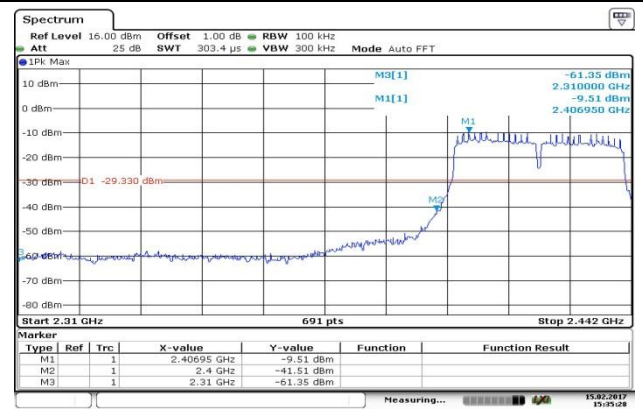
CH03-Bandedge
