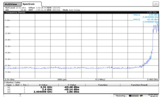
Bandedge- hopping mode (CH00)
