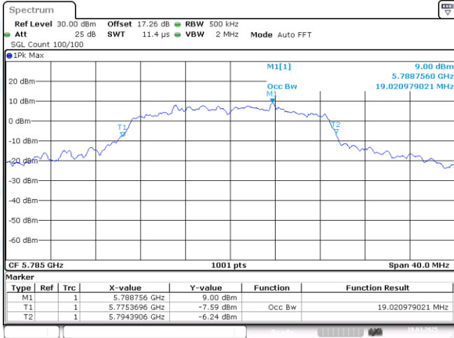
11N20MIMO-Ant2-5785
