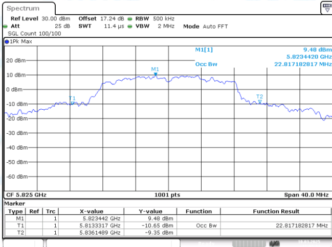
11A-Ant1-5825
