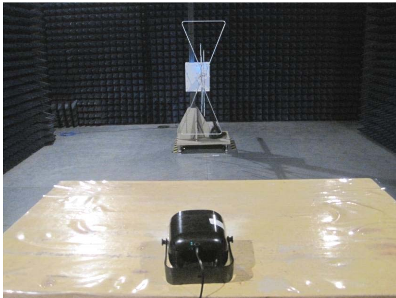
Photograph – Radiation Emission Test Setup
