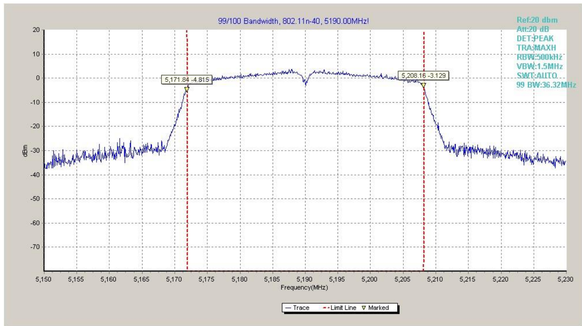
Fig. 98 99% Occupied bandwidth (802.11n40, 5190MHz)
