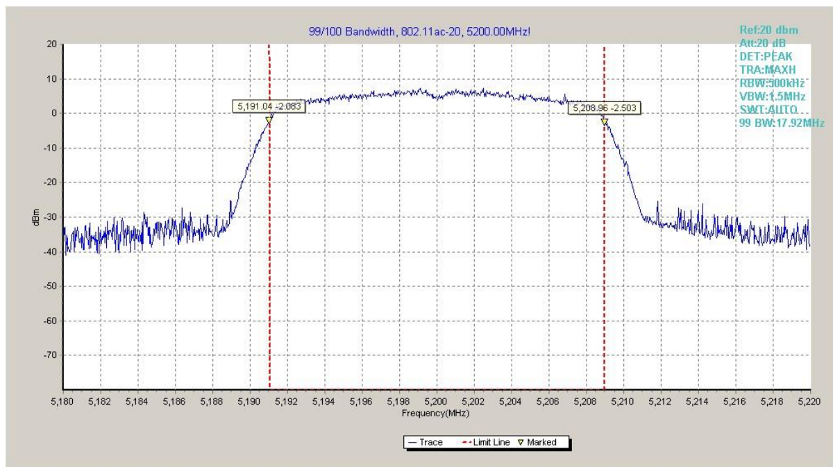
Fig. 96 99% Occupied bandwidth (802.11ac20, 5200MHz)
