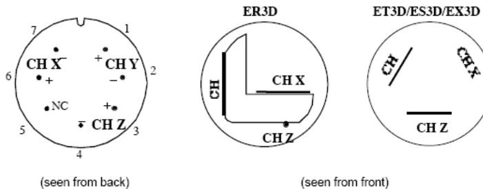
Connector Plan
