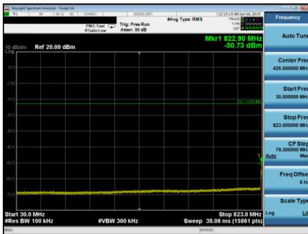
Plot 7-65. Conducted Spurious Plot (Band 5 - 10.0MHz QPSK - RB Size 1, RB Offset 0 - Low Channel)
