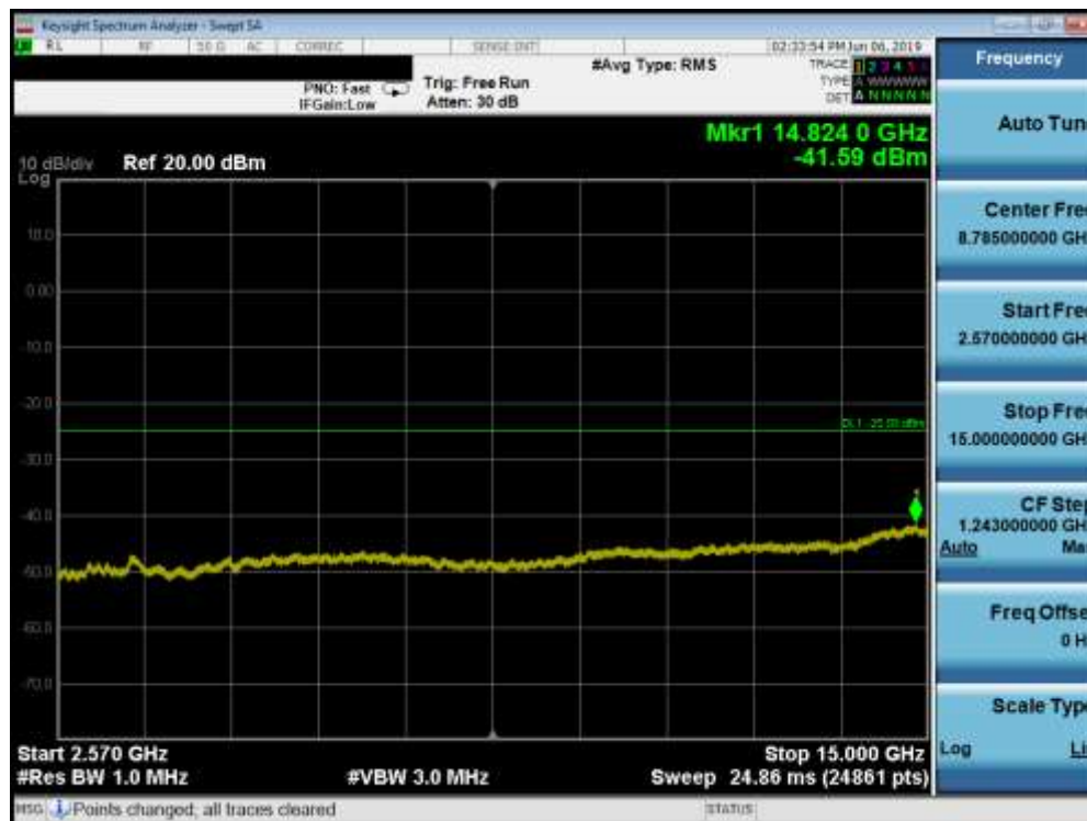
Plot 7-93. Conducted Spurious Plot (Band 7 - 20.0MHz QPSK - RB Size 1, RB Offset 0 - Low Channel)
