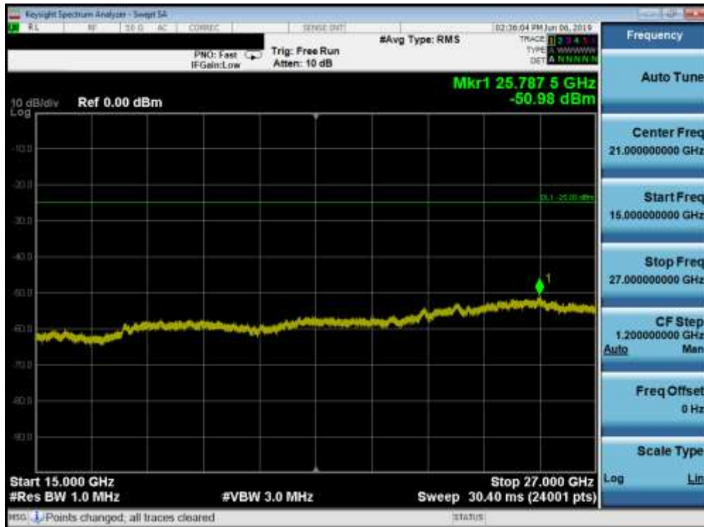
Plot 7-100. Conducted Spurious Plot (Band 7 - 20.0MHz QPSK - RB Size 1, RB Offset 0 - High Channel)
