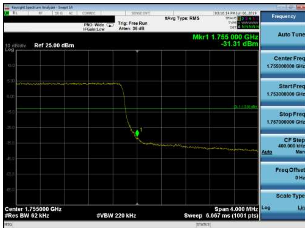
Plot 7-141. Upper Band Edge Plot (Band 4 - 5.0MHz QPSK - Full RB Configuration)
