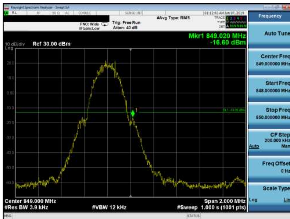
Plot 7-54. Band Edge Plot (Cell GPRS Mode - High Channel)
