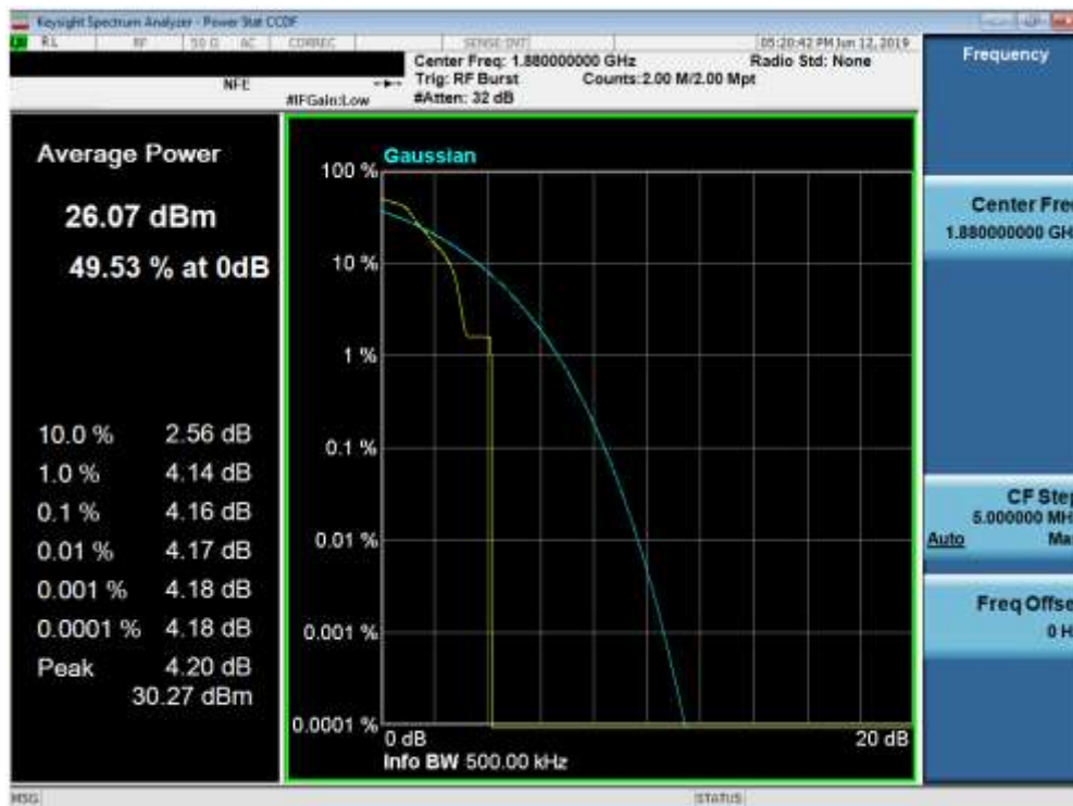
Plot 7-68. Peak-Average Ratio Plot (1900EDGE Mode)
