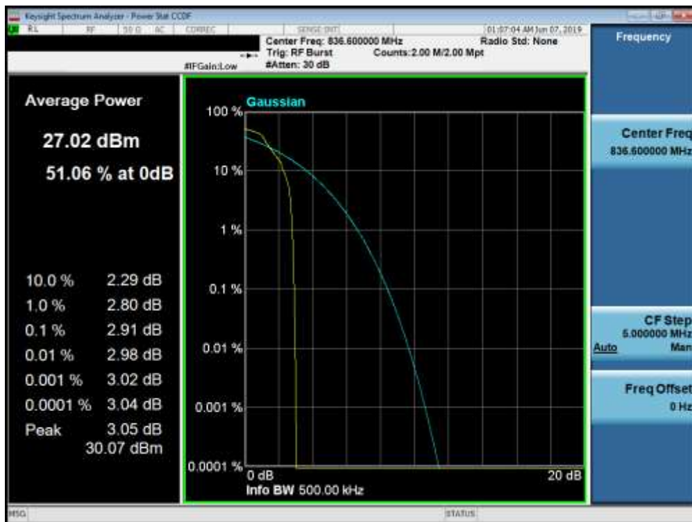
Plot 7-66. Peak-Average Ratio Plot (850EDGE Mode)
