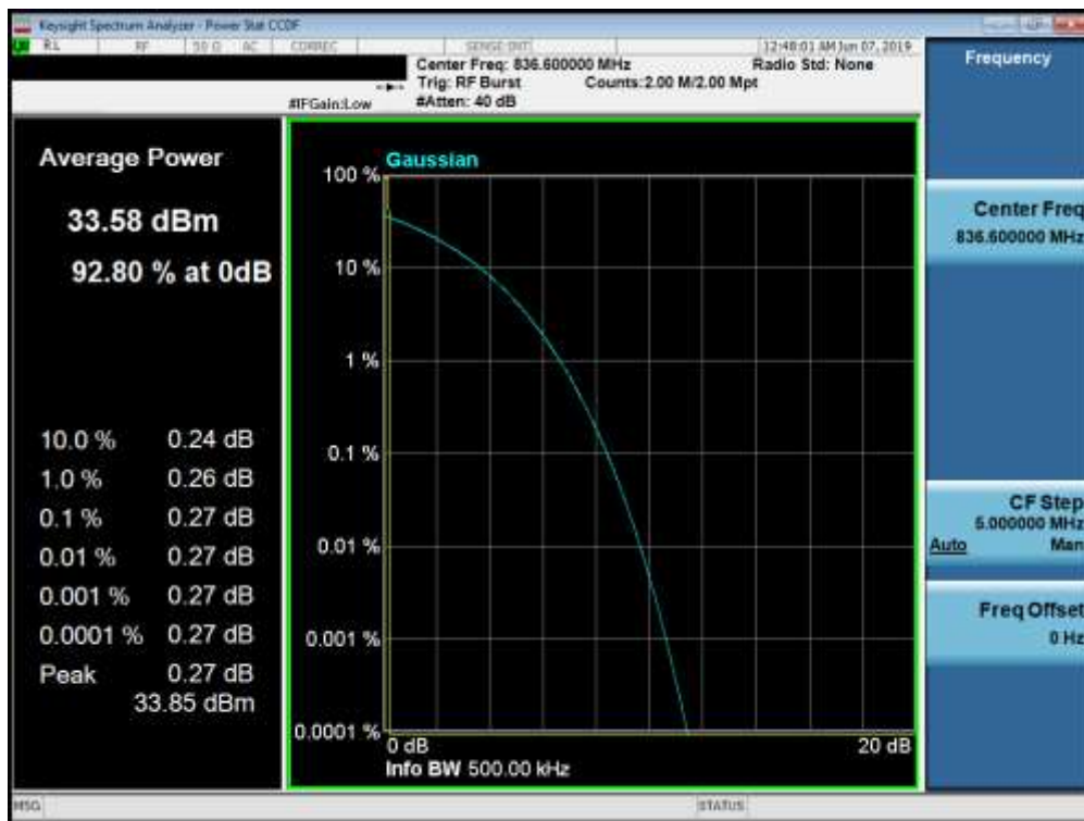
Plot 7-65. Peak-Average Ratio Plot (Cellular GPRS Mode)
