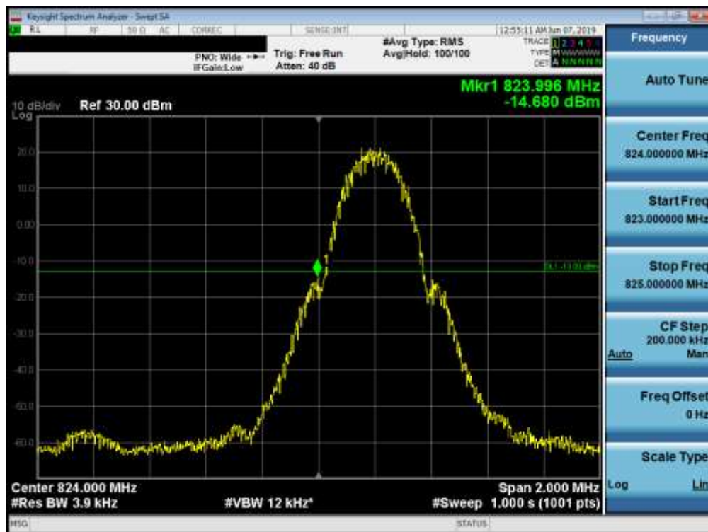
Plot 7-53. Band Edge Plot (Cell GPRS Mode - Low Channel)
