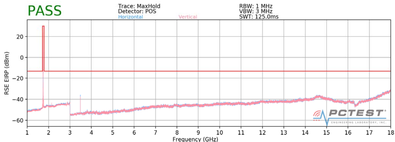
Plot 7-253. Radiated Spurious Plot above 1GHz (Band 66)
