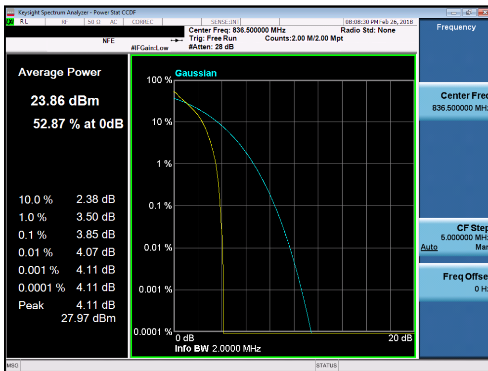
Plot 7-210. PAR Plot (Band 5 - 1.4MHz QPSK - Full RB Configuration)
