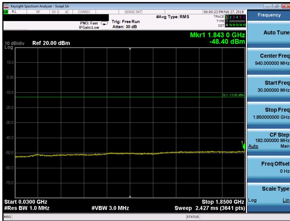
Plot 7-47. Conducted Spurious Plot (PCS WCDMA Mode - Mid Channel)
