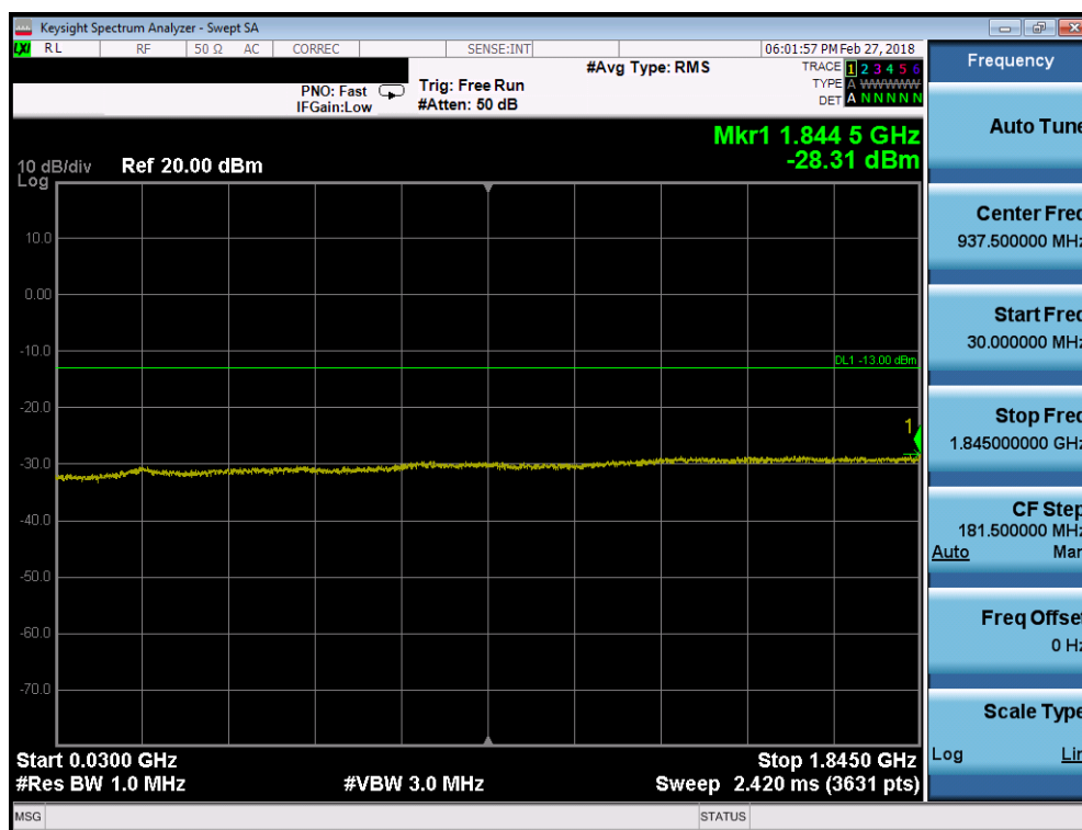
Plot 7-44. Conducted Spurious Plot (PCS WCDMA Mode - Low Channel)
