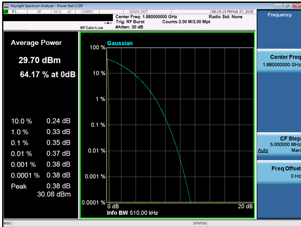
Plot 7-74. Peak-Average Ratio Plot (PCS GSM Mode)
