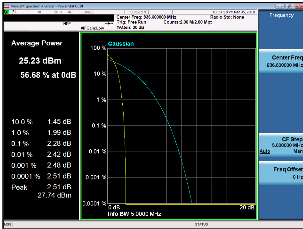
Plot 7-69. Peak-Average Ratio Plot (Cellular WCDMA Mode)
