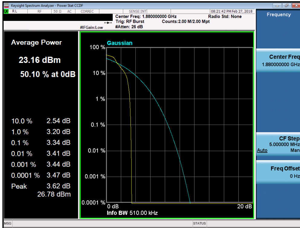
Plot 7-75. Peak-Average Ratio Plot (PCS EDGE Mode)
