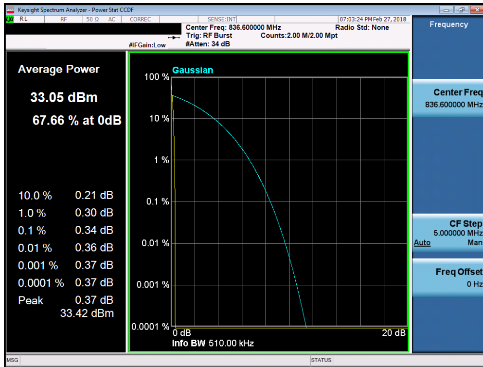
Plot 7-70. Peak-Average Ratio Plot (Cellular GSM Mode)
