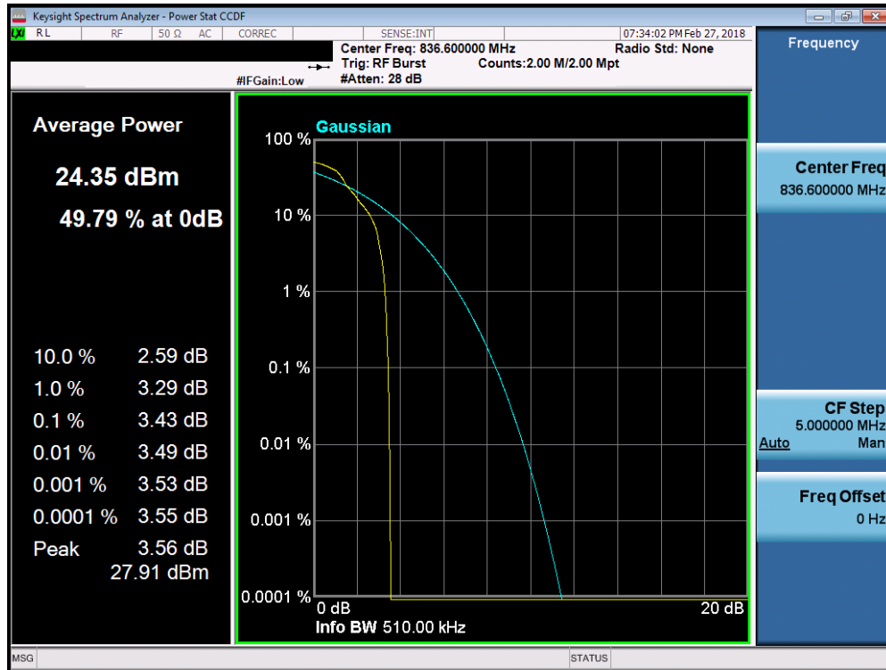
Plot 7-71. Peak-Average Ratio Plot (Cellular EDGE Mode)
