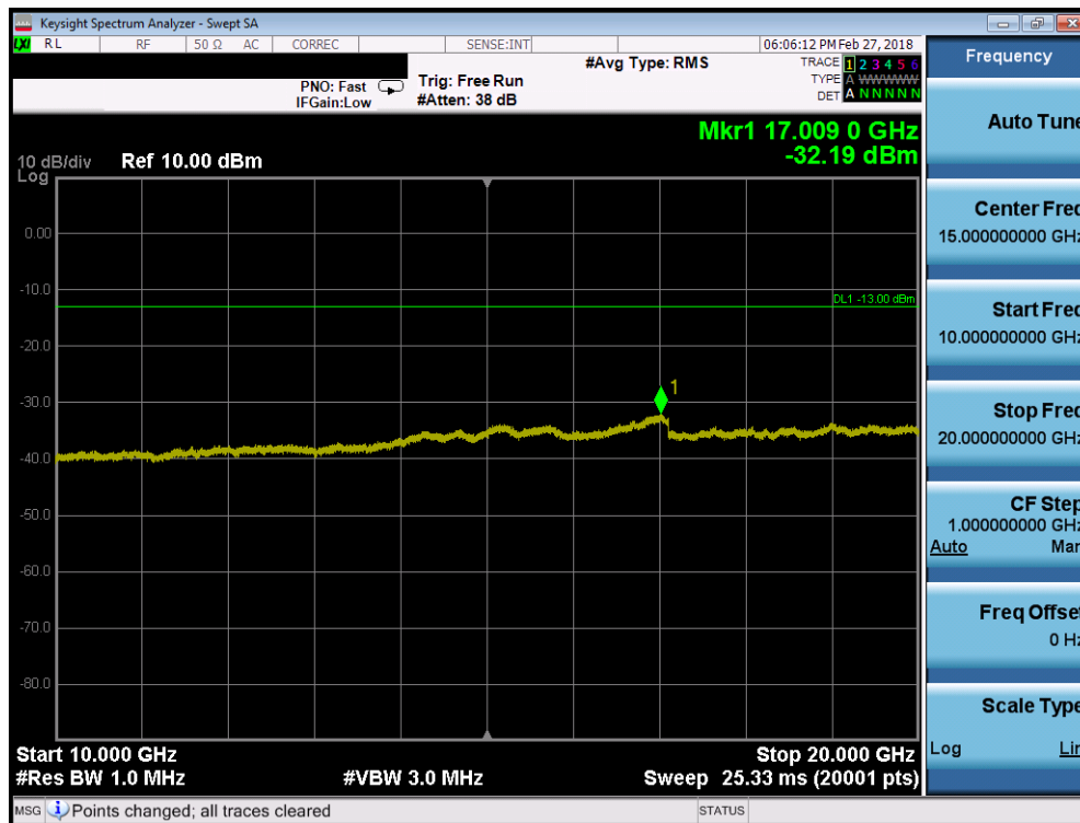
Plot 7-40. Conducted Spurious Plot (AWS WCDMA Mode - Mid Channel)
