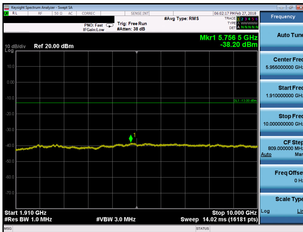
Plot 7-45. Conducted Spurious Plot (PCS WCDMA Mode - Low Channel)
