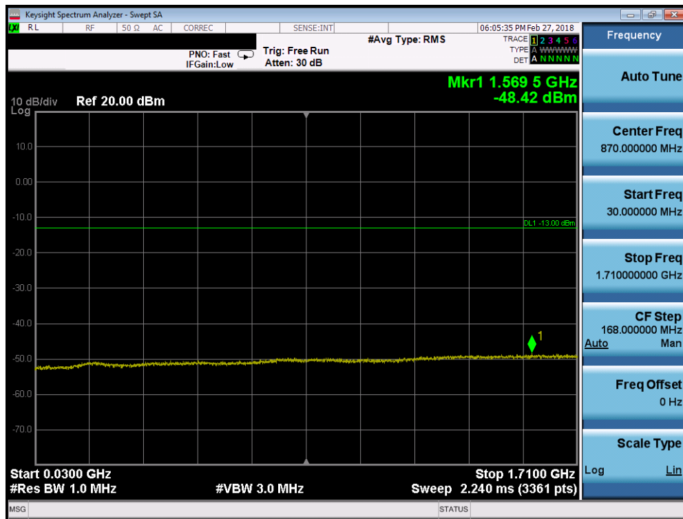
Plot 7-38. Conducted Spurious Plot (AWS WCDMA Mode - Mid Channel)
