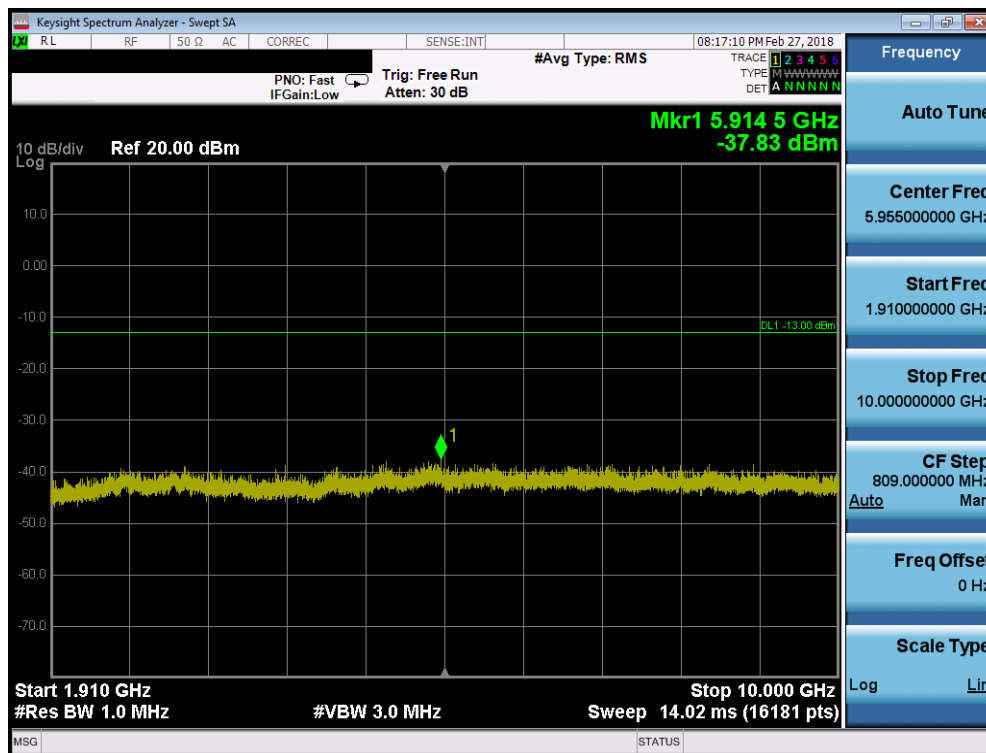
Plot 7-18. Conducted Spurious Plot (PCS GPRS Mode - Low Channel)
