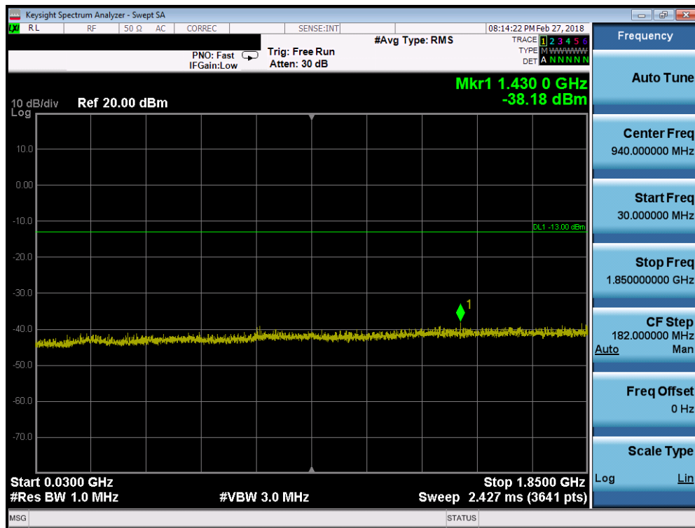
Plot 7-20. Conducted Spurious Plot (PCS GPRS Mode - Mid Channel)
