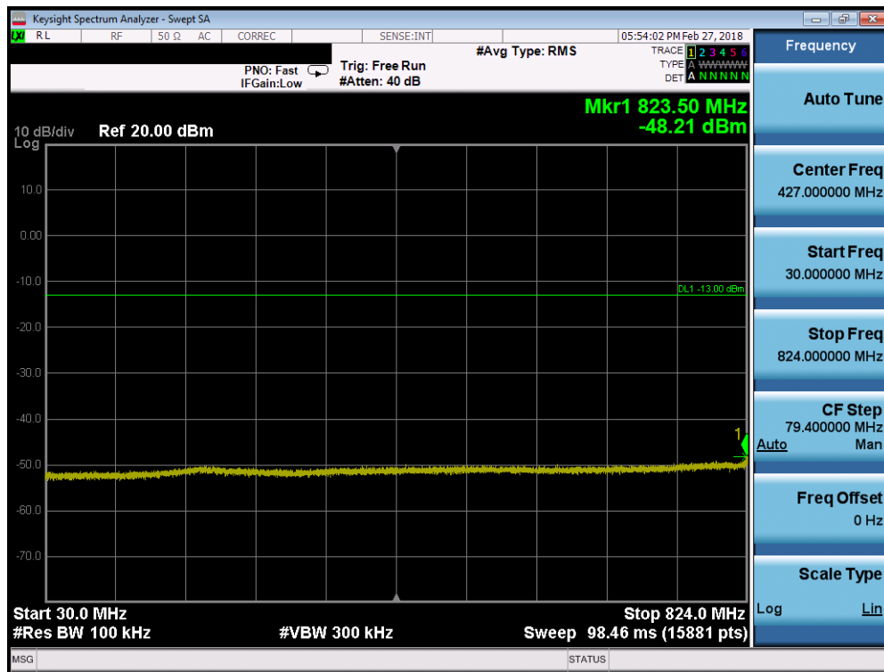
Plot 7-29. Conducted Spurious Plot (Cellular WCDMA Mode - Mid Channel)
