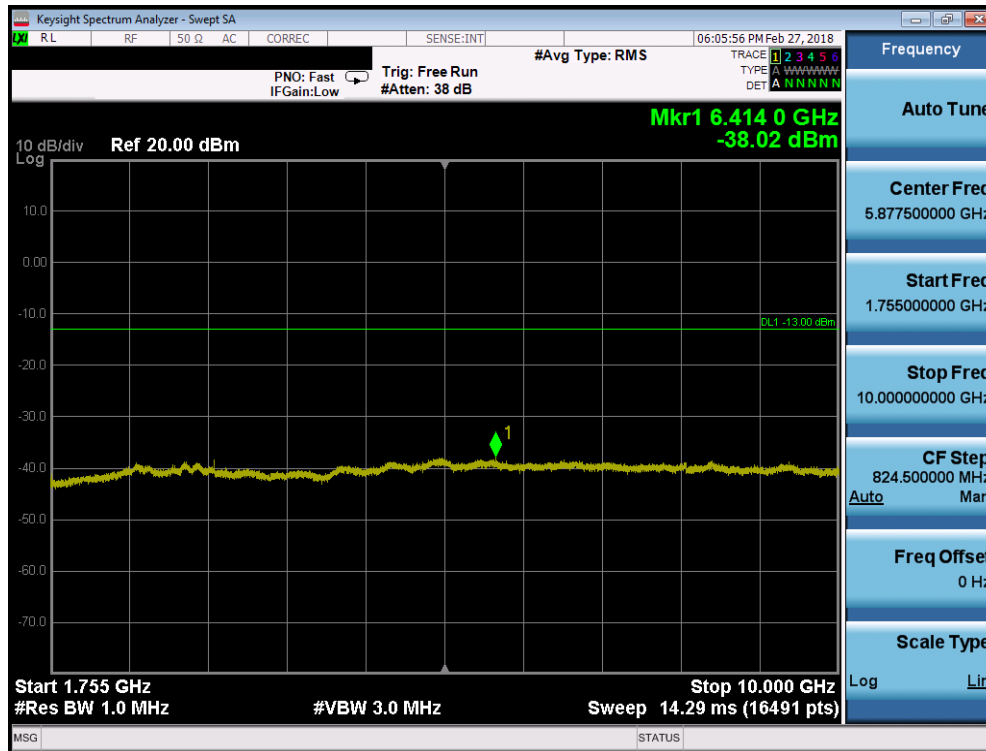
Plot 7-39. Conducted Spurious Plot (AWS WCDMA Mode - Mid Channel)
