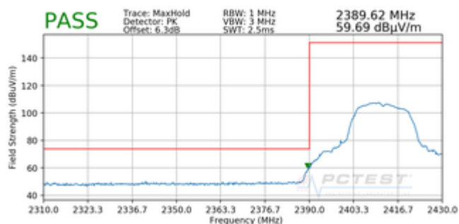
Plot 7-6. Radiated Restricted Lower Band Edge Measurement (Peak)
