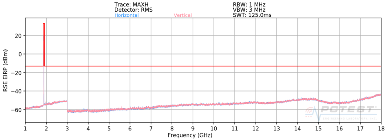
Plot 7-80. Radiated Spurious Plot above 1GHz (PCS WCDMA Mode)
