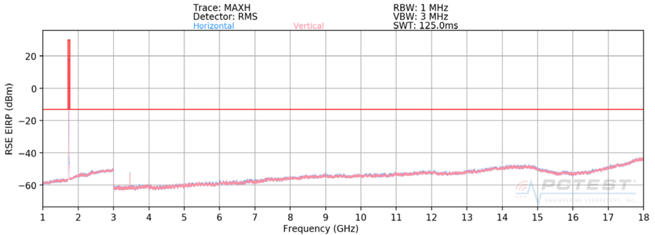
Plot 7-78. Radiated Spurious Plot above 1GHz (AWS WCDMA Mode)
