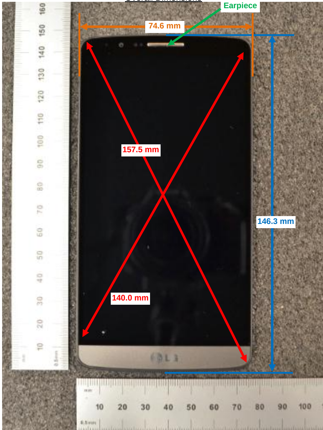
Overall Dimensions
