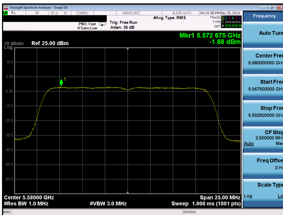
Plot 7-51. Power Spectral Density Plot (802.11a (UNII Band 2C) – Ch. 116)
