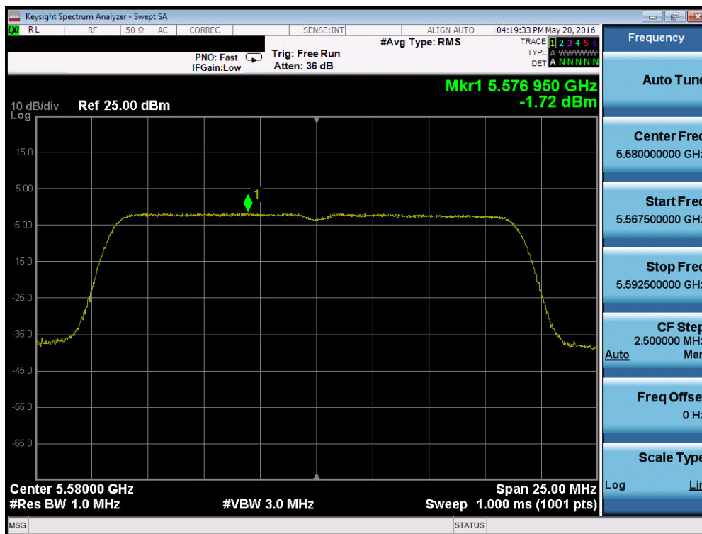
Plot 7-54. Power Spectral Density Plot (20MHz BW 802.11n (UNII Band 2C) – Ch. 116)
