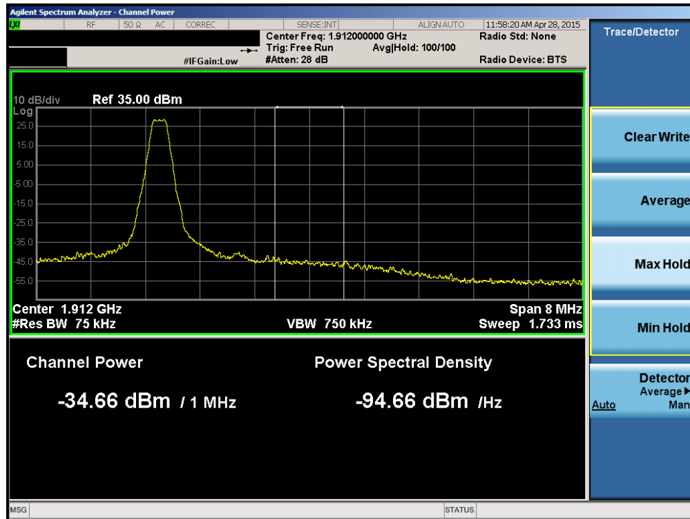
Plot 6-48. 8MHz Span Plot (PCS GSM Mode – Ch. 810)
