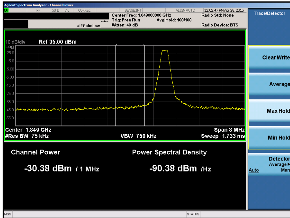
Plot 6-46. 8MHz Span Plot (PCS GSM Mode – Ch. 512)
