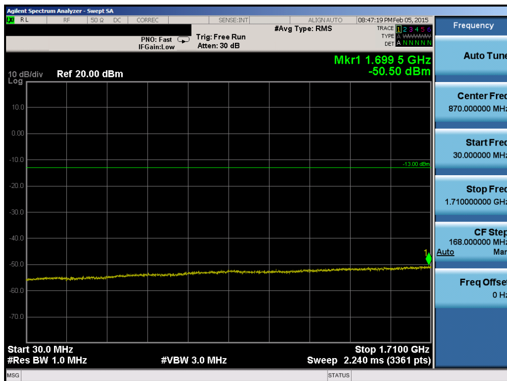
Plot 6-118. Conducted Spurious Plot (Band 4 – 10.0MHz QPSK – RB Size 1, RB Offset 0 – High Channel)
