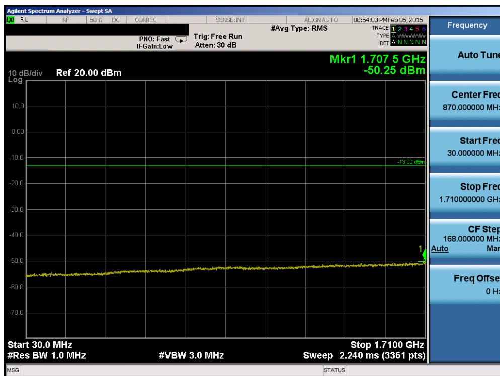
Plot 6-124. Conducted Spurious Plot (Band 4 – 15.0MHz QPSK – RB Size 1, RB Offset 0 – Mid Channel)
