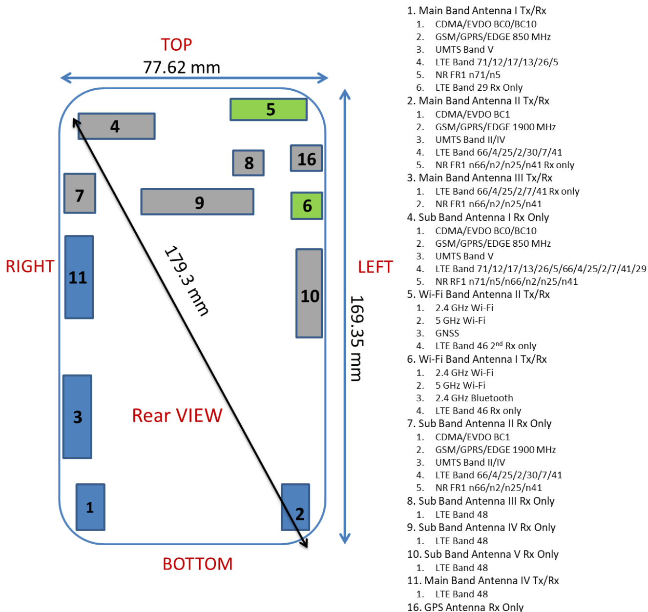
Figure E-1 DUT Antenna Locations
