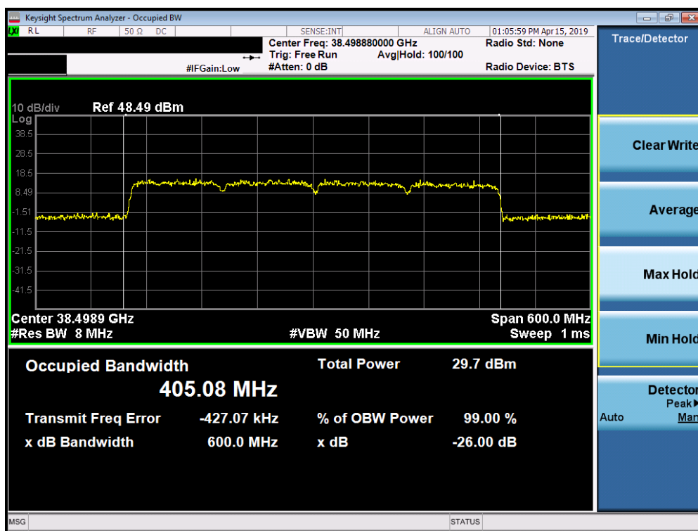
Plot 7-24. Occupied Bandwidth Plot (4CC-100MHz Bandwidth 64QAM Mid Channel)
