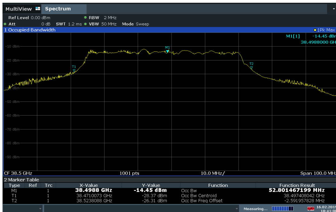
Plot 7-37. Occupied Bandwidth Plot (1CC-50MHz Bandwidth QPSK Mid Channel)
