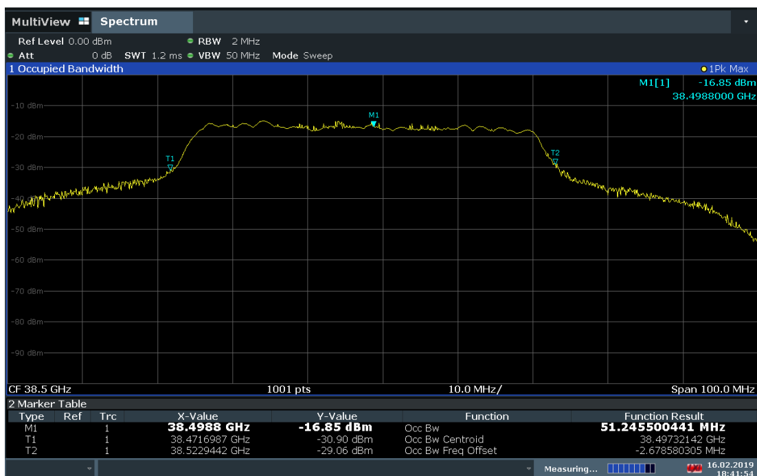
Plot 7-39. Occupied Bandwidth Plot (1CC-50MHz Bandwidth 64QAM Mid Channel)
