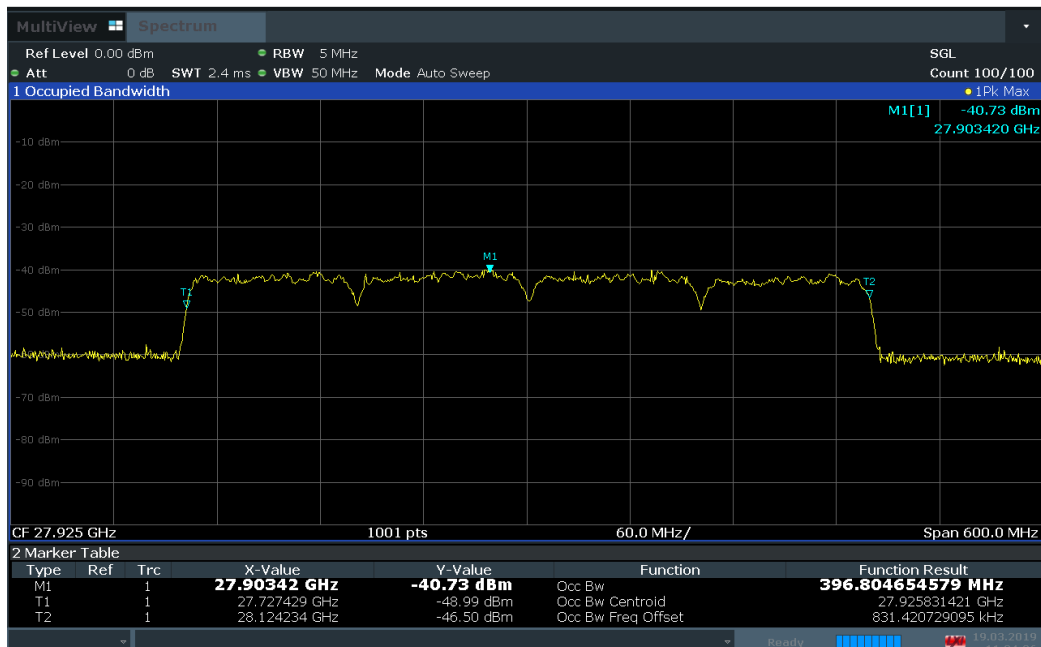
Plot 7-35. Occupied Bandwidth Plot (4CC-100MHz Bandwidth 16QAM Mid Channel)
