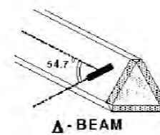
Figure F.2.1 Triangular Probe Configurations
