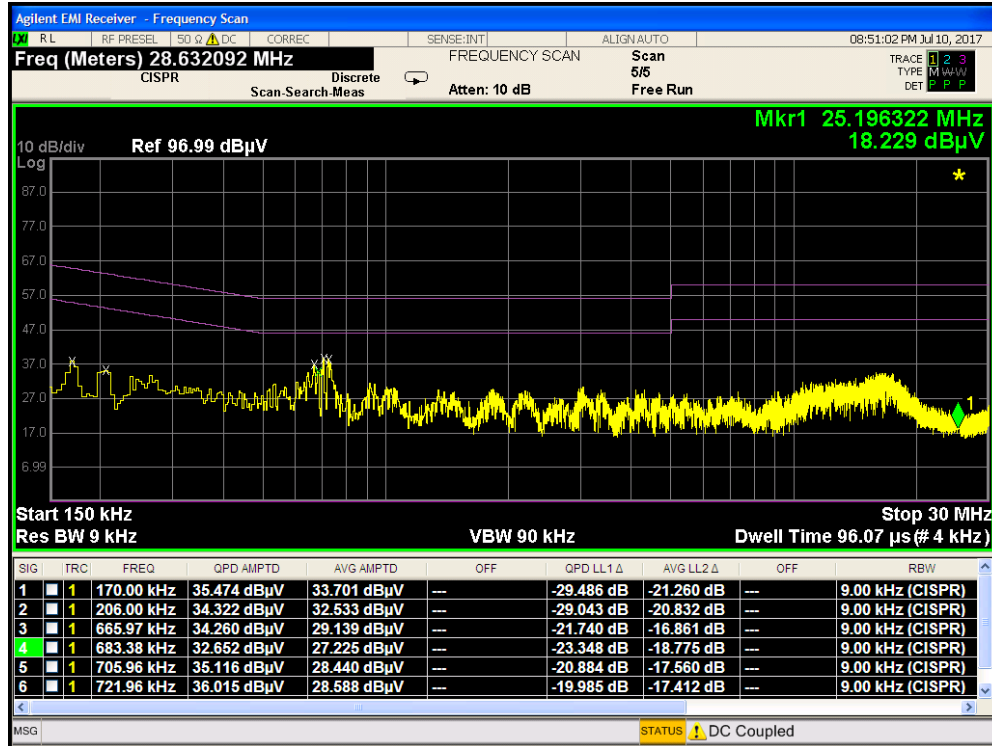
Plot 7-8. Line-Conducted Test Plot with NFC antenna terminated (L1)
