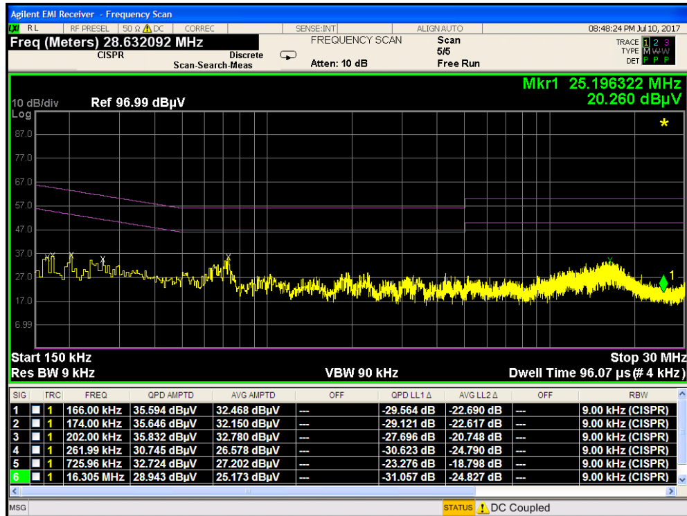
Plot 7-9. Line-Conducted Test Plot with NFC antenna terminated (N)
