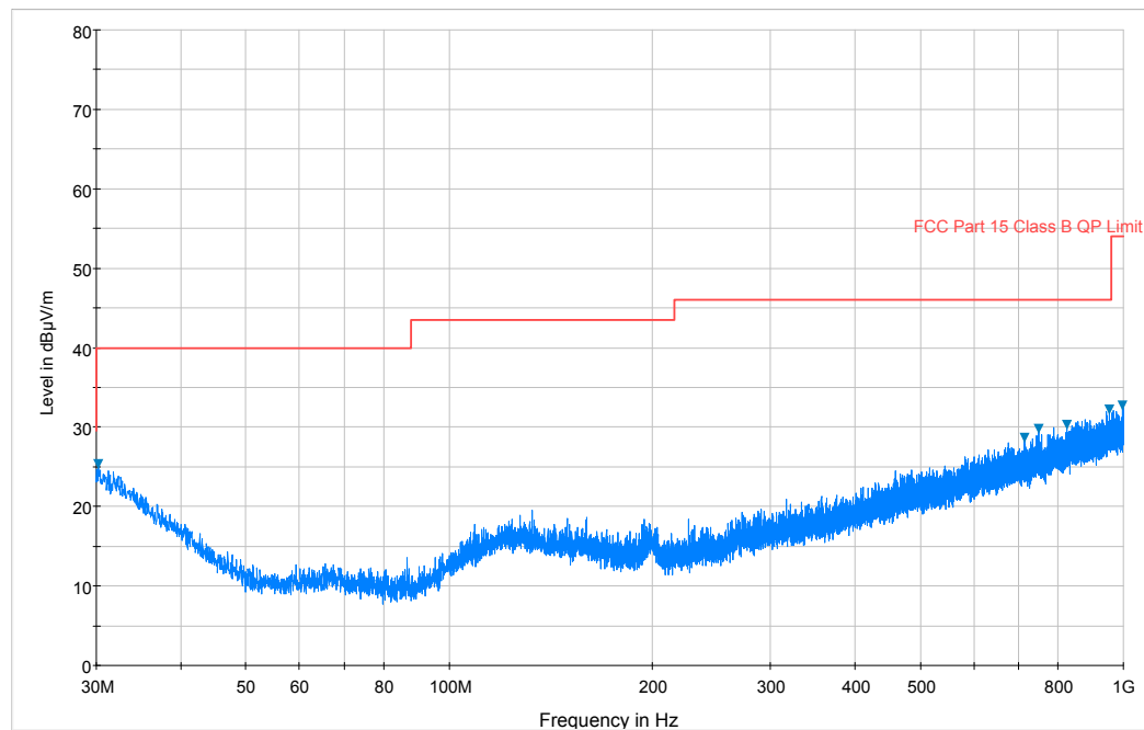
Plot 7-4. Radiated Spurious Plot 30MHz – 1GHz (Pol. H)
