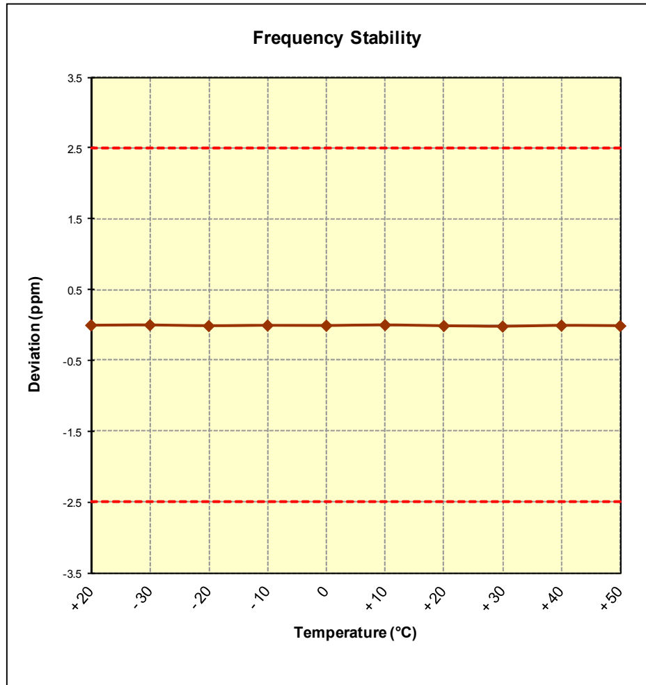
Figure 6-7. Frequency Stability Graph (Cellular CDMA Mode – Ch. 384)
