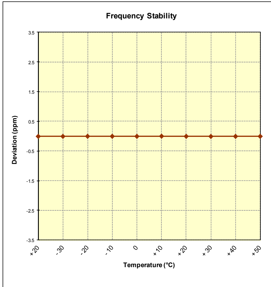
Figure 6-8. Frequency Stability Graph (PCS CDMA Mode – Ch. 600)
