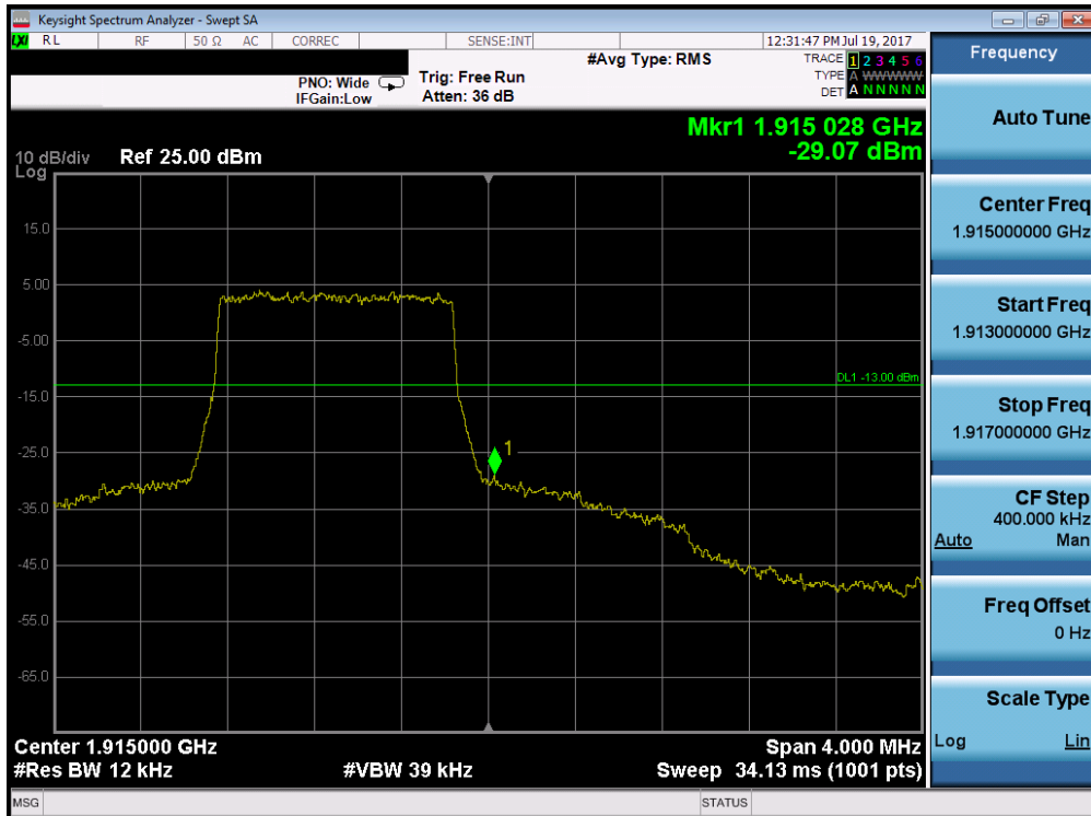
Plot 7-171. Upper Band Edge Plot (Band 25 – 1.4MHz QPSK – RB Size 6)
