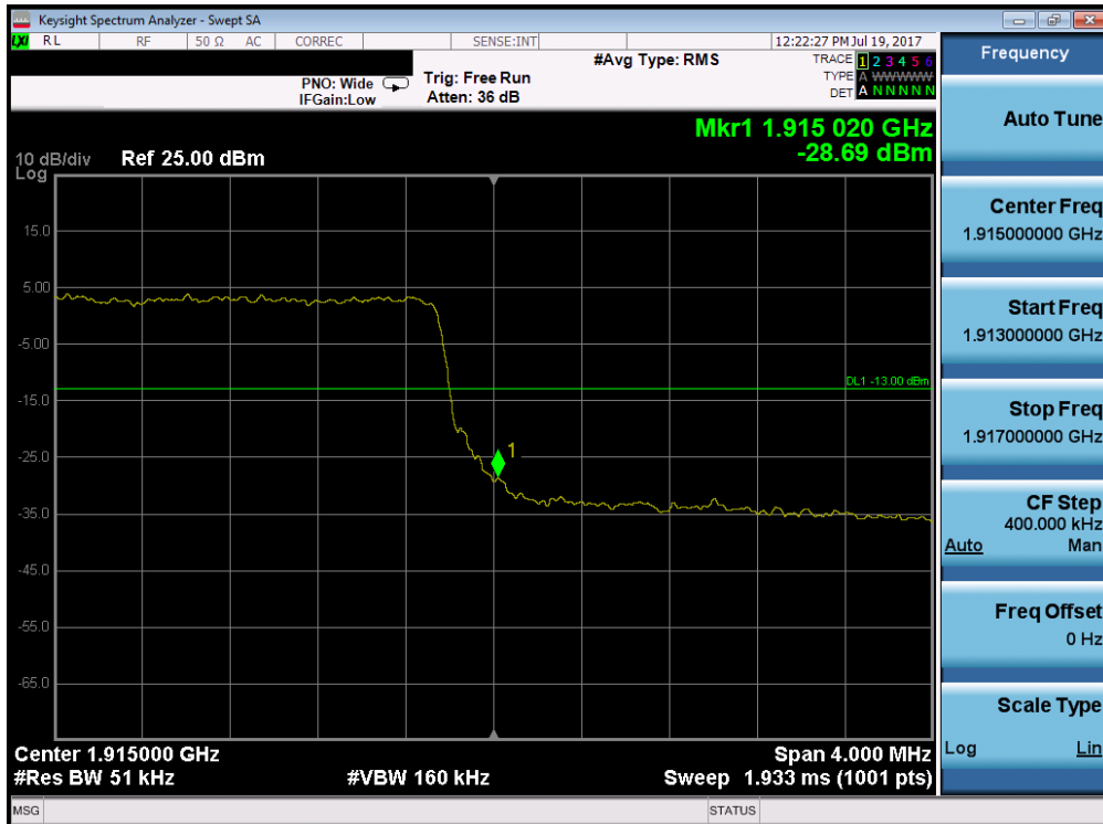
Plot 7-179. Upper Band Edge Plot (Band 25 – 5.0MHz QPSK – RB Size 25)
