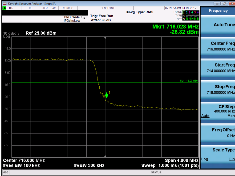
Plot 7-114. Upper Band Edge Plot (Band 12 – 5.0MHz QPSK – RB Size 25)
