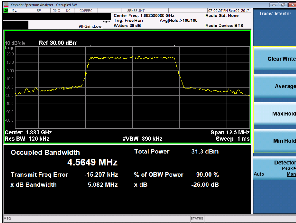
Plot 7-41. Occupied Bandwidth Plot (Band 25/2 - 5.0MHz QPSK - Full RB Configuration)
