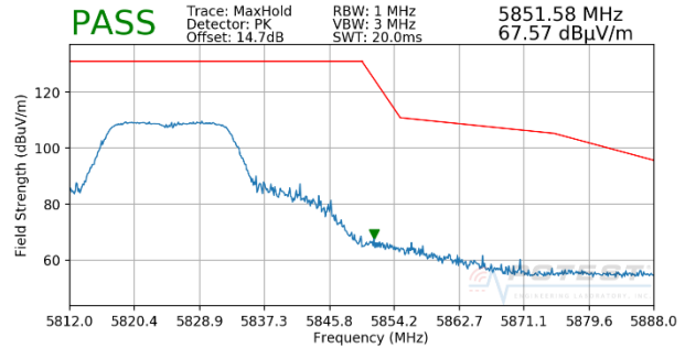
Plot 7-100. Radiated Upper Band Edge Plot (Peak – UNII Band 3)
