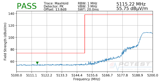
Plot 7-86. Radiated Lower Band Edge Plot (Peak – UNII Band 1 - Interior)
