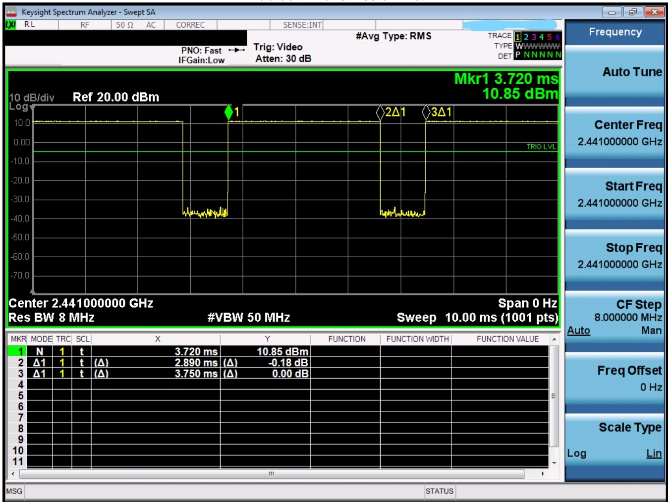
Equation 9-1 Bluetooth Duty Cycle Calculation
