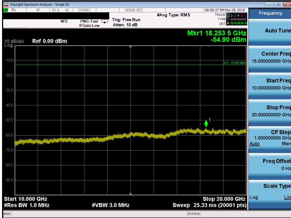
Plot 7-80. Conducted Spurious Plot (Band 2 - 1.4MHz QPSK - RB Size 1, RB Offset 0 - High Channel)
