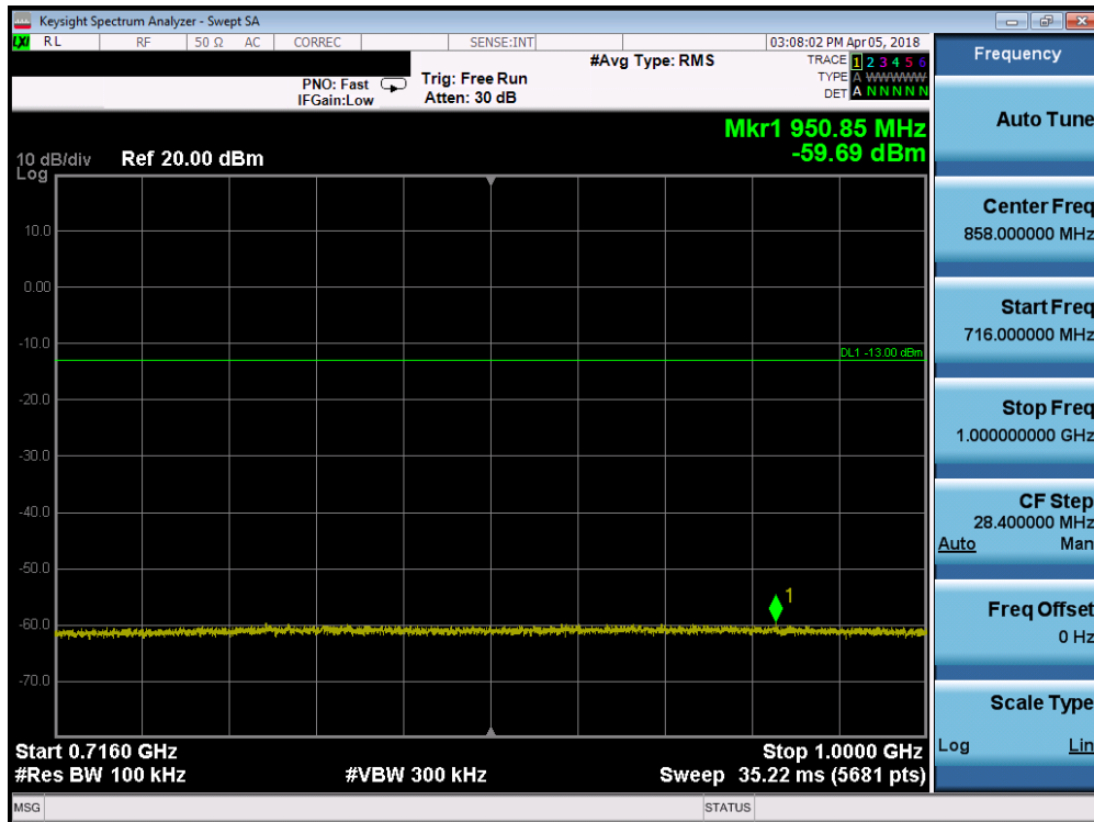
Plot 7-46. Conducted Spurious Plot (Band 12 - 1.4MHz QPSK - RB Size 1, RB Offset 0 - Low Channel)
