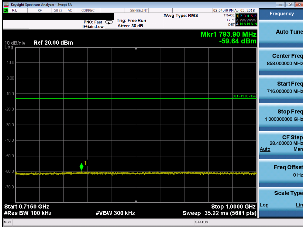
Plot 7-49. Conducted Spurious Plot (Band 12 - 1.4MHz QPSK - RB Size 1, RB Offset 0 - Mid Channel)
