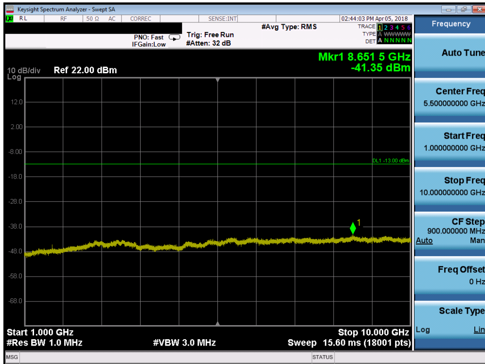
Plot 7-56. Conducted Spurious Plot (Band 5 - 1.4MHz QPSK - RB Size 1, RB Offset 0 - Low Channel)
