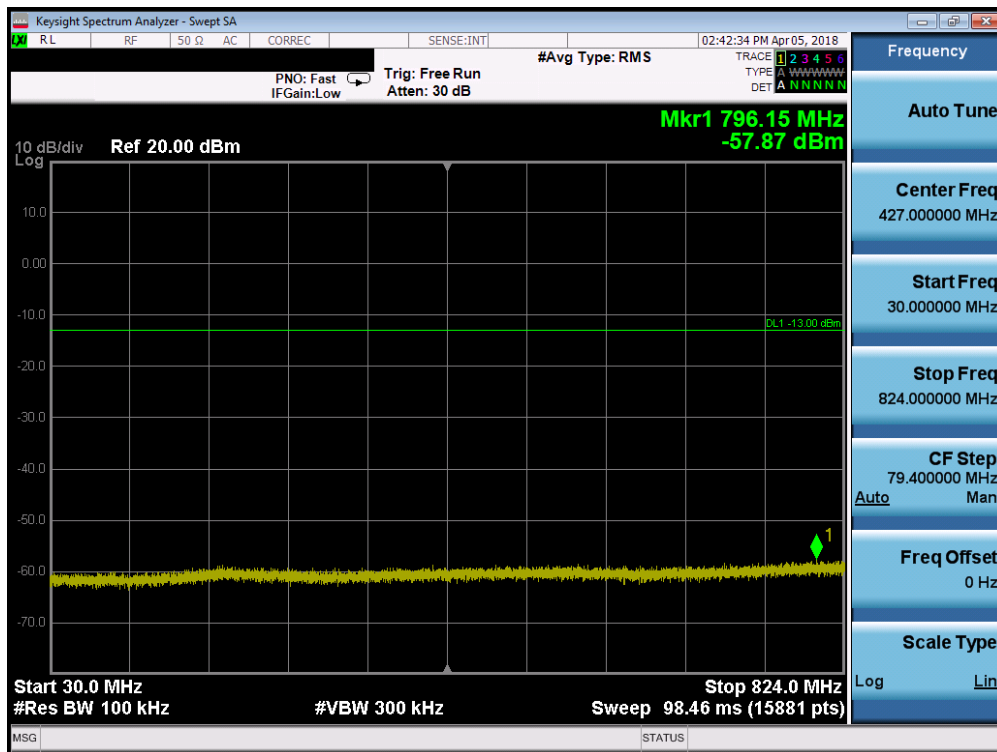
Plot 7-57. Conducted Spurious Plot (Band 5 - 1.4MHz QPSK - RB Size 1, RB Offset 0 - Mid Channel)
