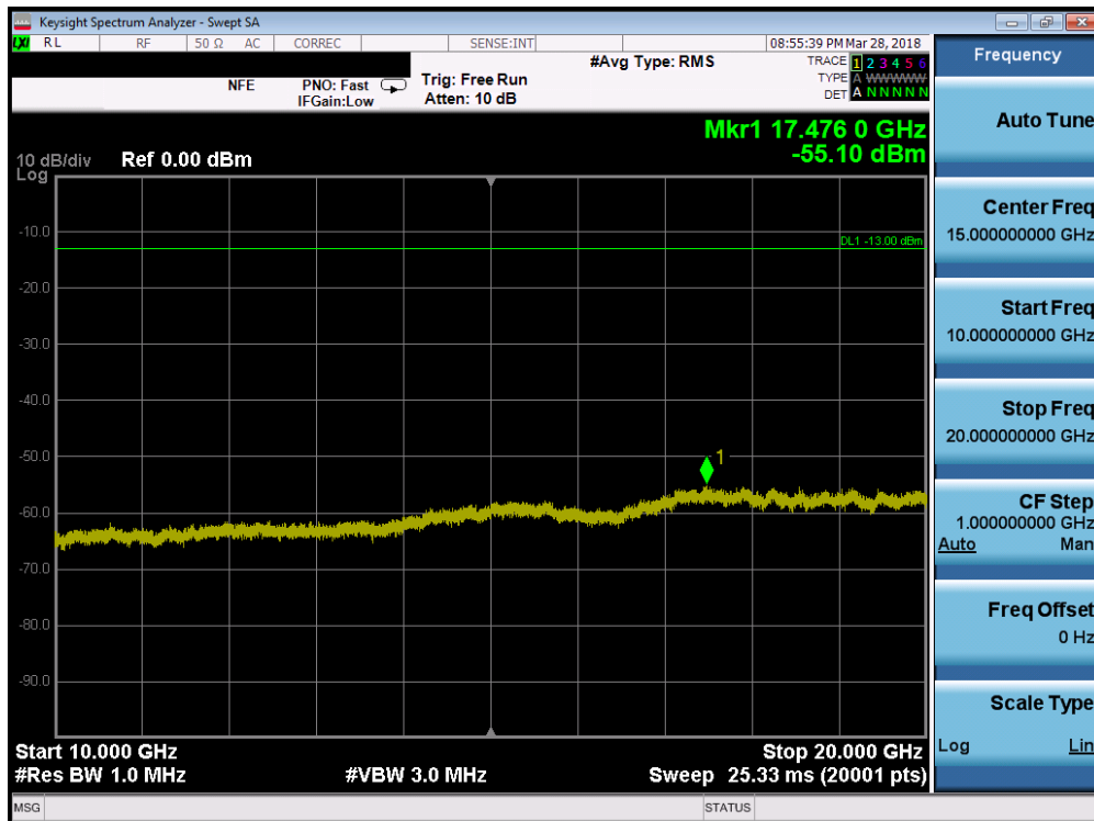
Plot 7-77. Conducted Spurious Plot (Band 2 - 1.4MHz QPSK - RB Size 1, RB Offset 0 - Mid Channel)
