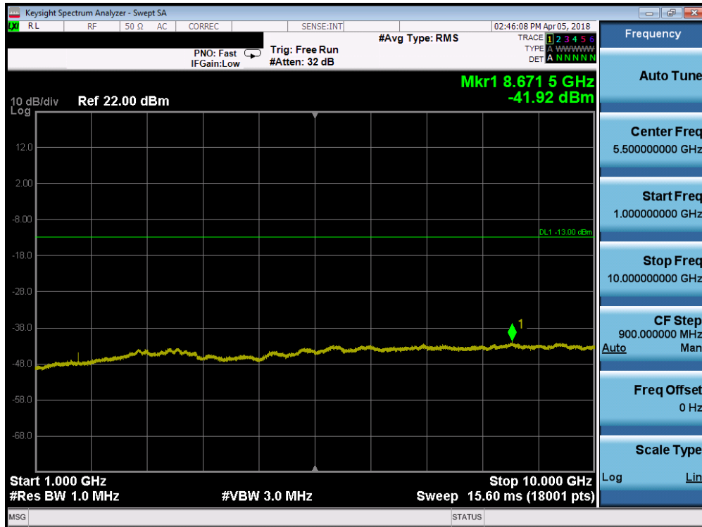
Plot 7-62. Conducted Spurious Plot (Band 5 - 1.4MHz QPSK - RB Size 1, RB Offset 0 - High Channel)
