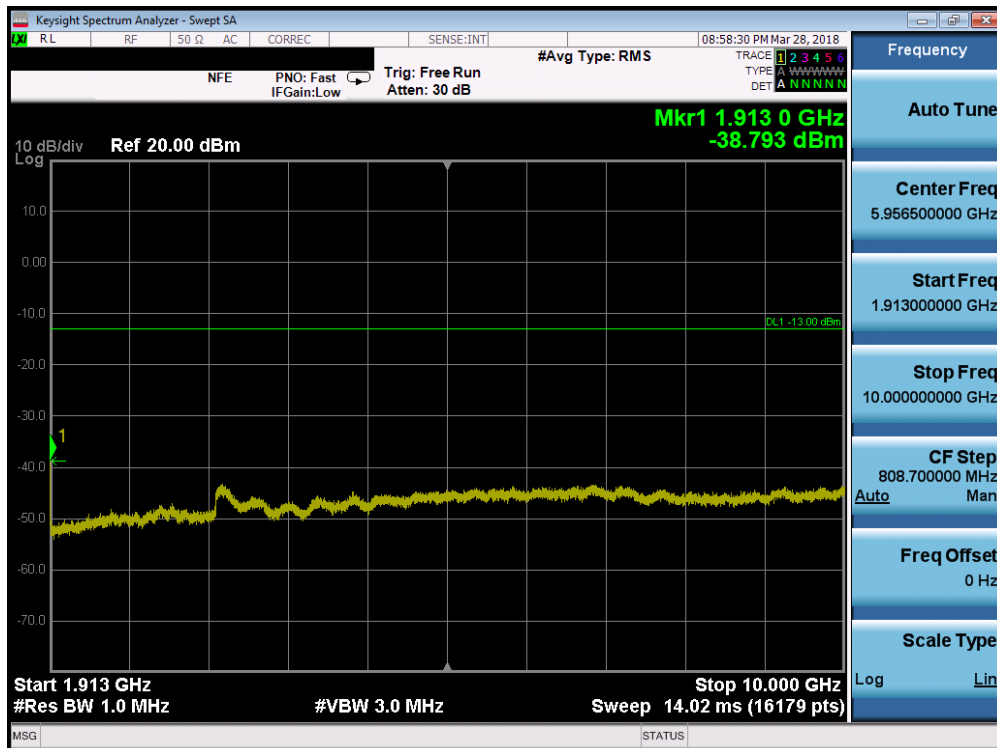
Plot 7-79. Conducted Spurious Plot (Band 2 - 1.4MHz QPSK - RB Size 1, RB Offset 0 - High Channel)
