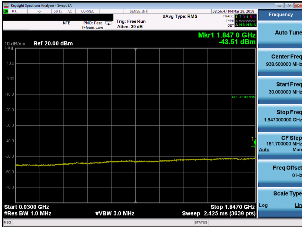
Plot 7-72. Conducted Spurious Plot (Band 2 - 1.4MHz QPSK - RB Size 1, RB Offset 0 - Low Channel)
