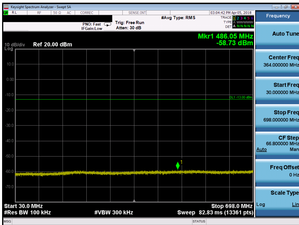
Plot 7-48. Conducted Spurious Plot (Band 12 - 1.4MHz QPSK - RB Size 1, RB Offset 0 - Mid Channel)
