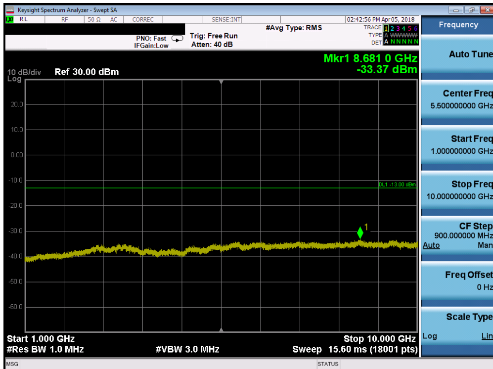
Plot 7-59. Conducted Spurious Plot (Band 5 - 1.4MHz QPSK - RB Size 1, RB Offset 0 - Mid Channel)
