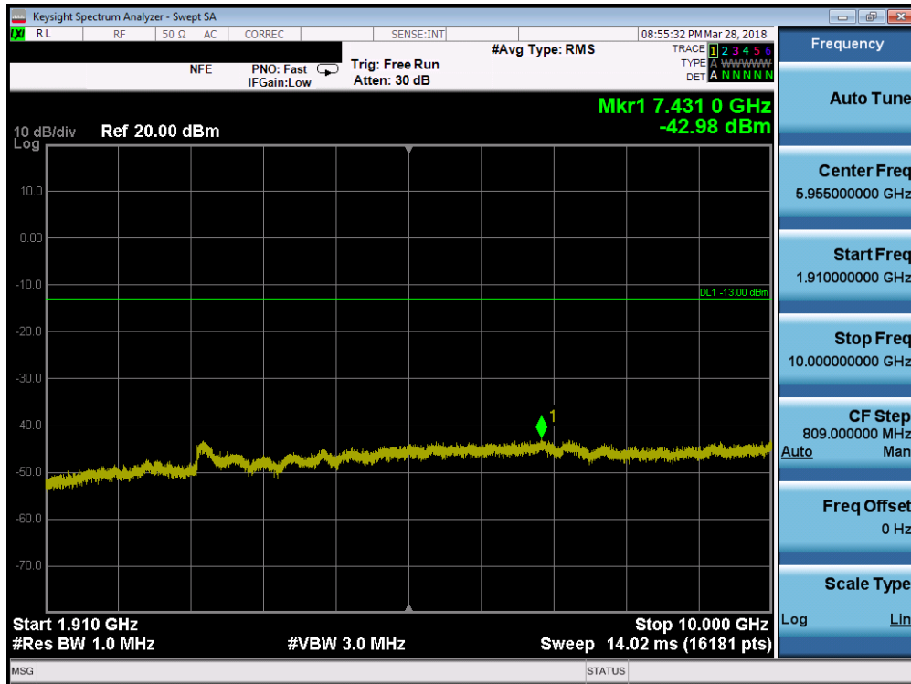
Plot 7-76. Conducted Spurious Plot (Band 2 - 1.4MHz QPSK - RB Size 1, RB Offset 0 - Mid Channel)
