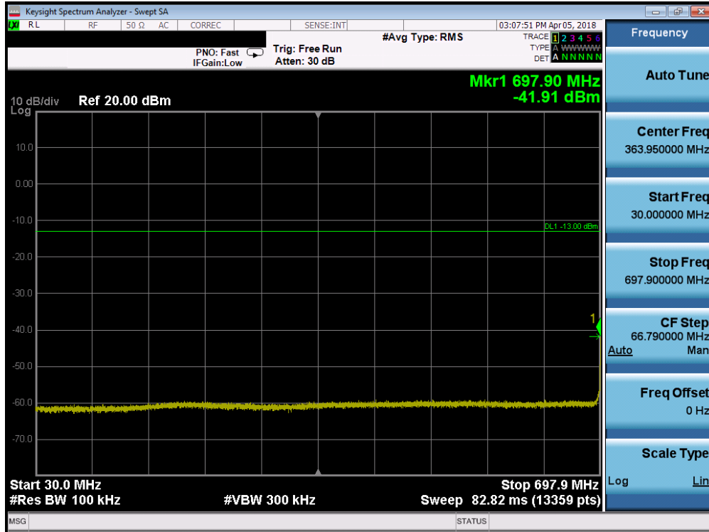
Plot 7-45. Conducted Spurious Plot (Band 12 - 1.4MHz QPSK - RB Size 1, RB Offset 0 - Low Channel)
