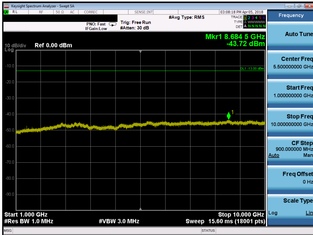
Plot 7-47. Conducted Spurious Plot (Band 12 - 1.4MHz QPSK - RB Size 1, RB Offset 0 - Low Channel)
