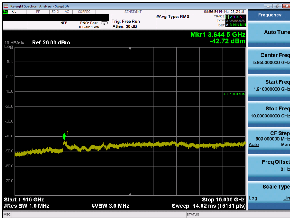
Plot 7-73. Conducted Spurious Plot (Band 2 - 1.4MHz QPSK - RB Size 1, RB Offset 0 - Low Channel)
