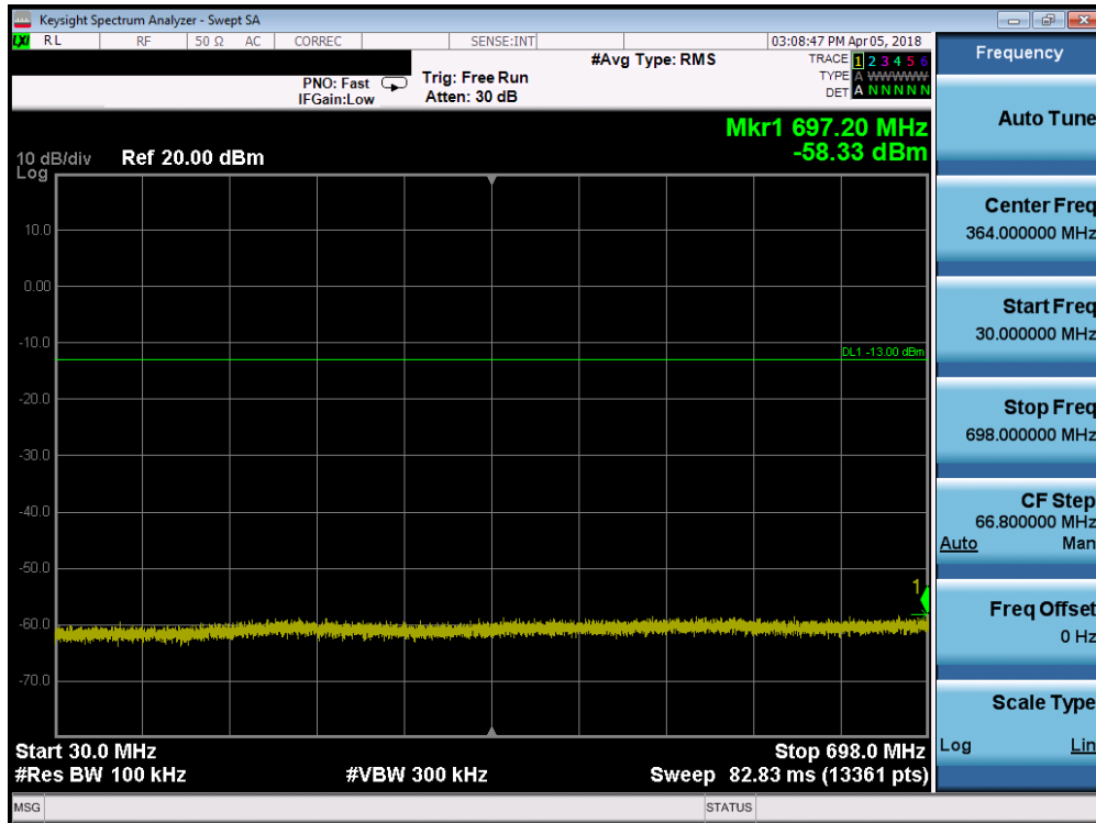
Plot 7-51. Conducted Spurious Plot (Band 12 - 1.4MHz QPSK - RB Size 1, RB Offset 0 - High Channel)
