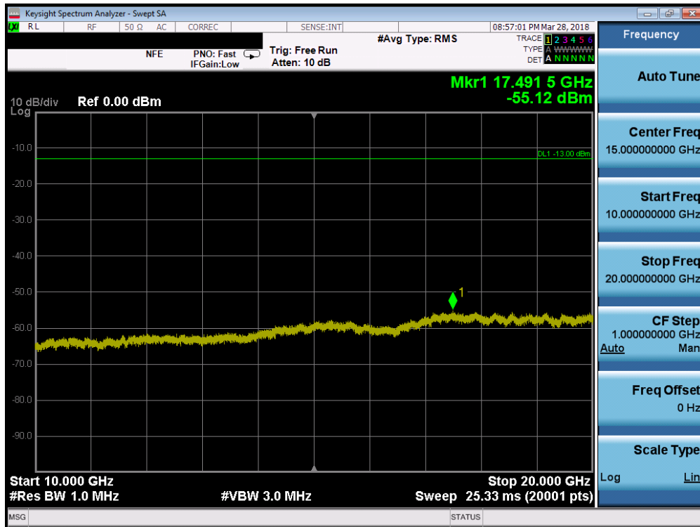
Plot 7-74. Conducted Spurious Plot (Band 2 - 1.4MHz QPSK - RB Size 1, RB Offset 0 - Low Channel)
