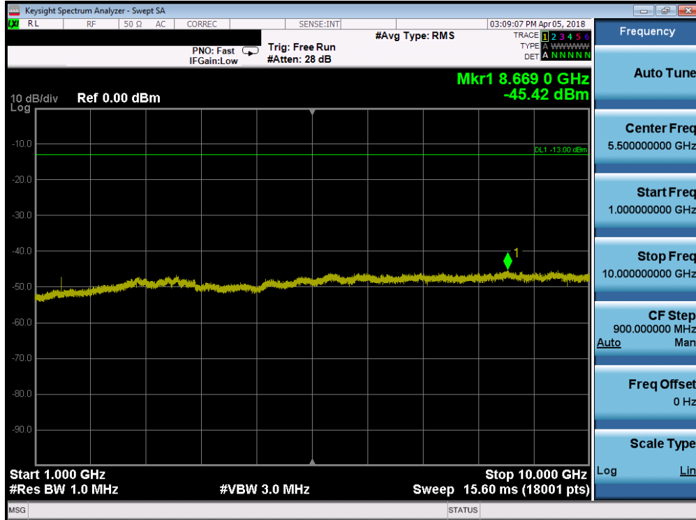
Plot 7-53. Conducted Spurious Plot (Band 12 - 1.4MHz QPSK - RB Size 1, RB Offset 0 - High Channel)
