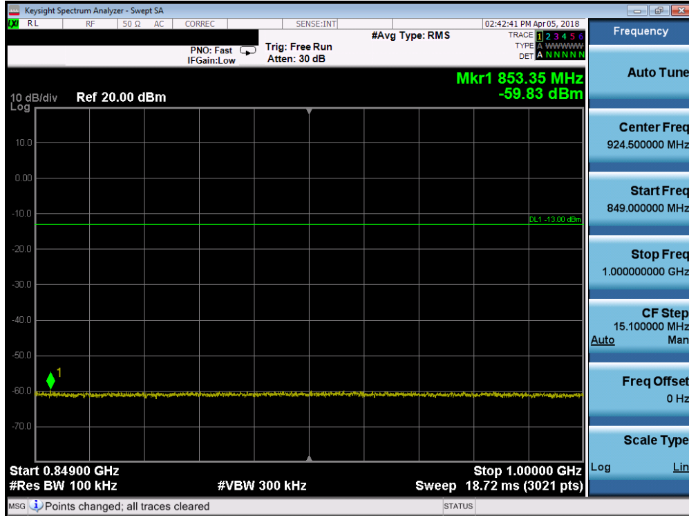
Plot 7-58. Conducted Spurious Plot (Band 5 - 1.4MHz QPSK - RB Size 1, RB Offset 0 - Mid Channel)
