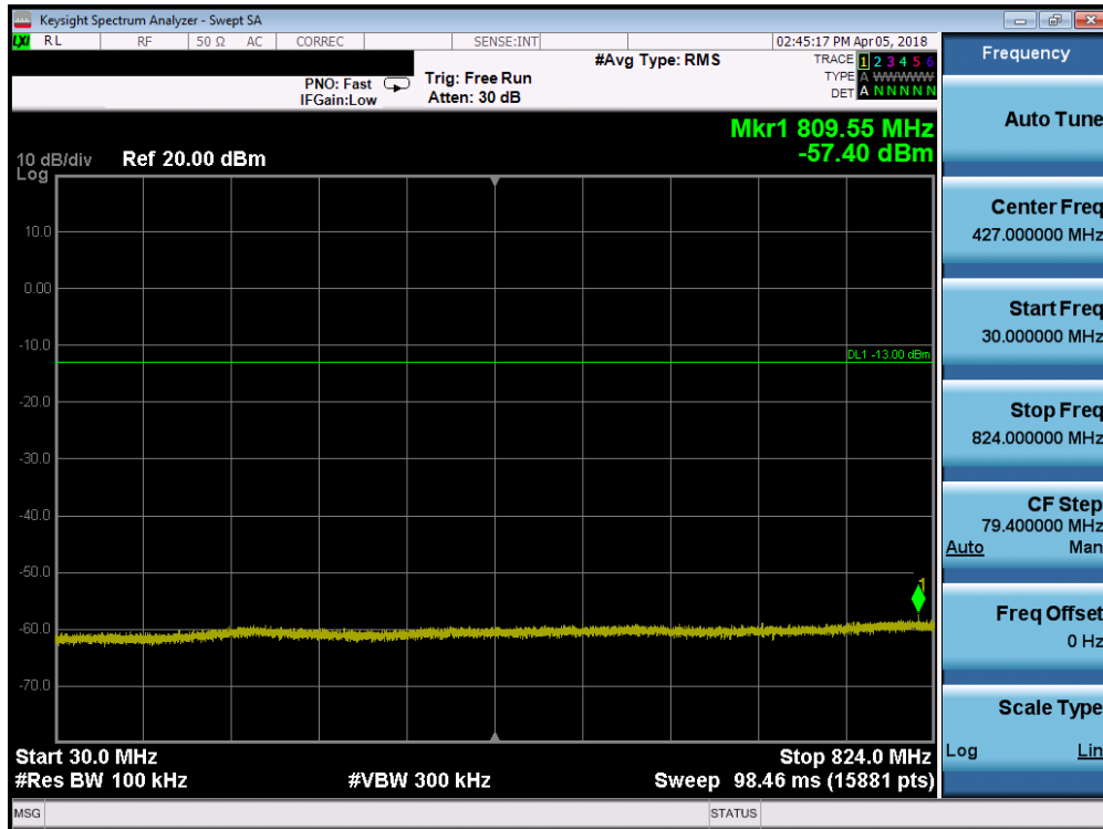
Plot 7-60. Conducted Spurious Plot (Band 5 - 1.4MHz QPSK - RB Size 1, RB Offset 0 - High Channel)
