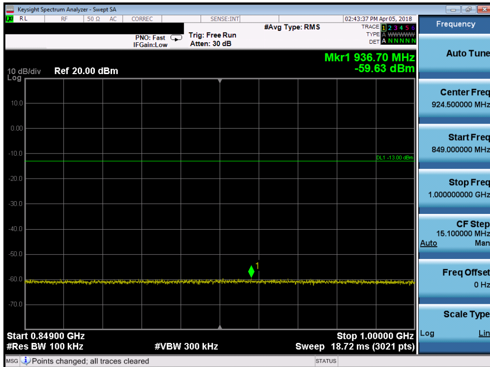
Plot 7-55. Conducted Spurious Plot (Band 5 - 1.4MHz QPSK - RB Size 1, RB Offset 0 - Low Channel)
