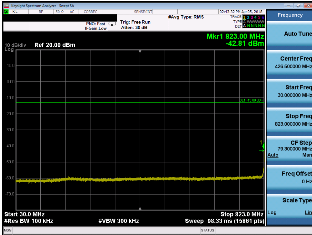
Plot 7-54. Conducted Spurious Plot (Band 5 - 1.4MHz QPSK - RB Size 1, RB Offset 0 - Low Channel)
