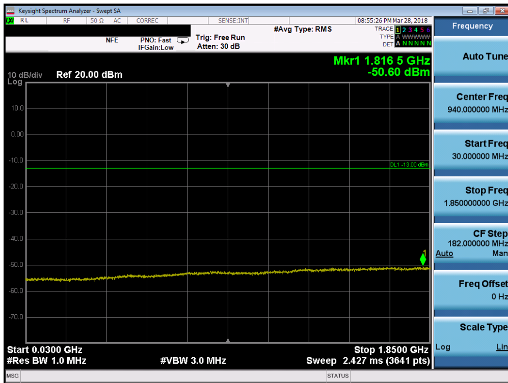
Plot 7-75. Conducted Spurious Plot (Band 2 - 1.4MHz QPSK - RB Size 1, RB Offset 0 - Mid Channel)
