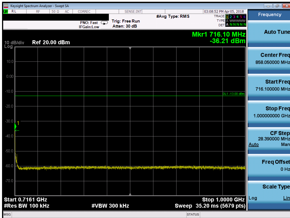
Plot 7-52. Conducted Spurious Plot (Band 12 - 1.4MHz QPSK - RB Size 1, RB Offset 0 - High Channel)
