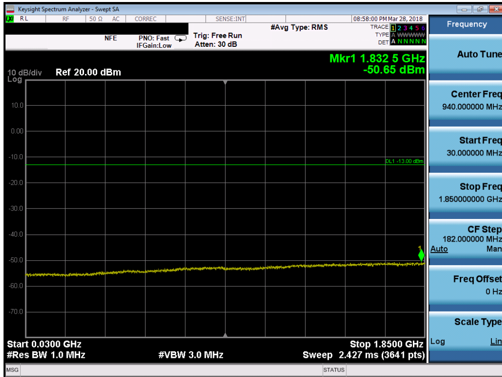
Plot 7-78. Conducted Spurious Plot (Band 2 - 1.4MHz QPSK - RB Size 1, RB Offset 0 - High Channel)
