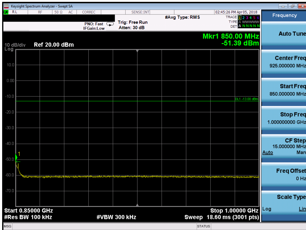
Plot 7-61. Conducted Spurious Plot (Band 5 - 1.4MHz QPSK - RB Size 1, RB Offset 0 - High Channel)
