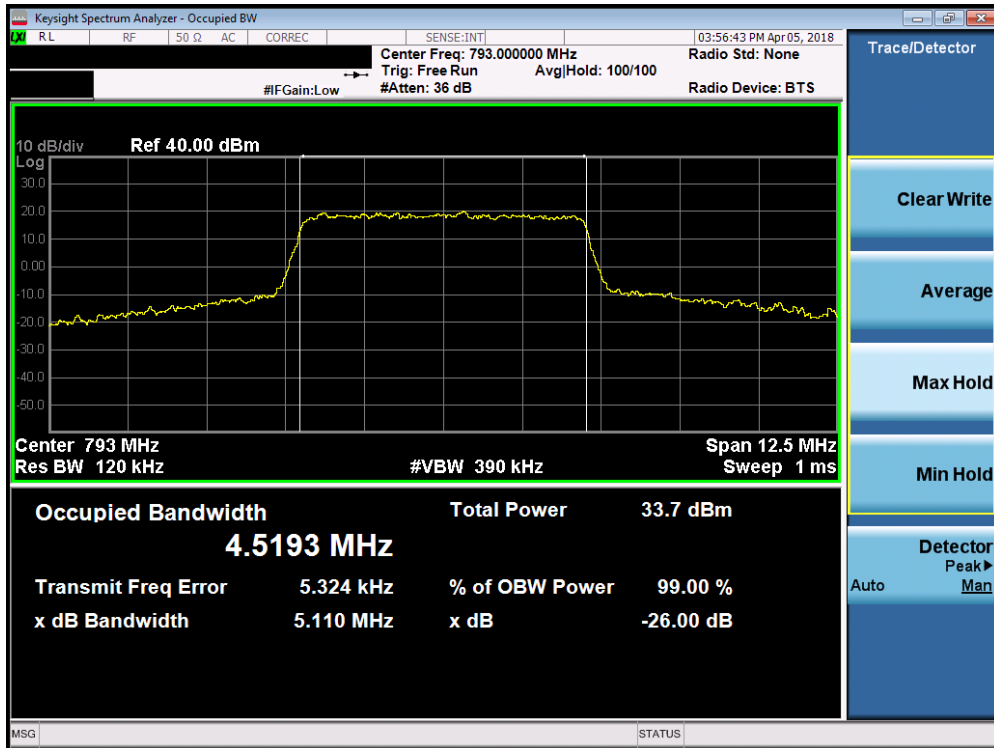
Plot 7-1. Occupied Bandwidth Plot (Band 14 - 5.0MHz QPSK - Full RB Configuration)
