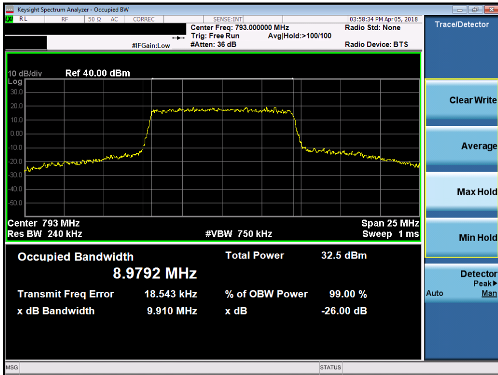
Plot 7-4. Occupied Bandwidth Plot (Band 14 - 10.0MHz 16-QAM - Full RB Configuration)
