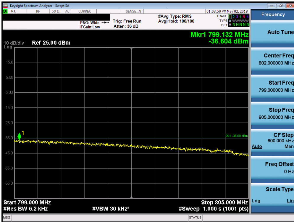
Plot 7-15. Upper Emission Mask Band Edge Plot (Band 14 - 10.0MHz QPSK - Full RB Configuration)
