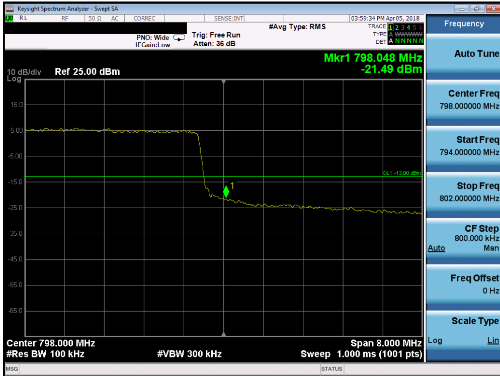
Plot 7-14. Upper Band Edge Plot (Band 14 - 10.0MHz QPSK - Full RB Configuration)
