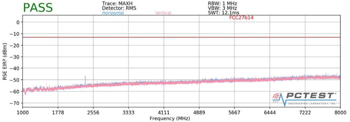
Plot 7-16. Radiated Spurious Plot above 1GHz (Band 14)
