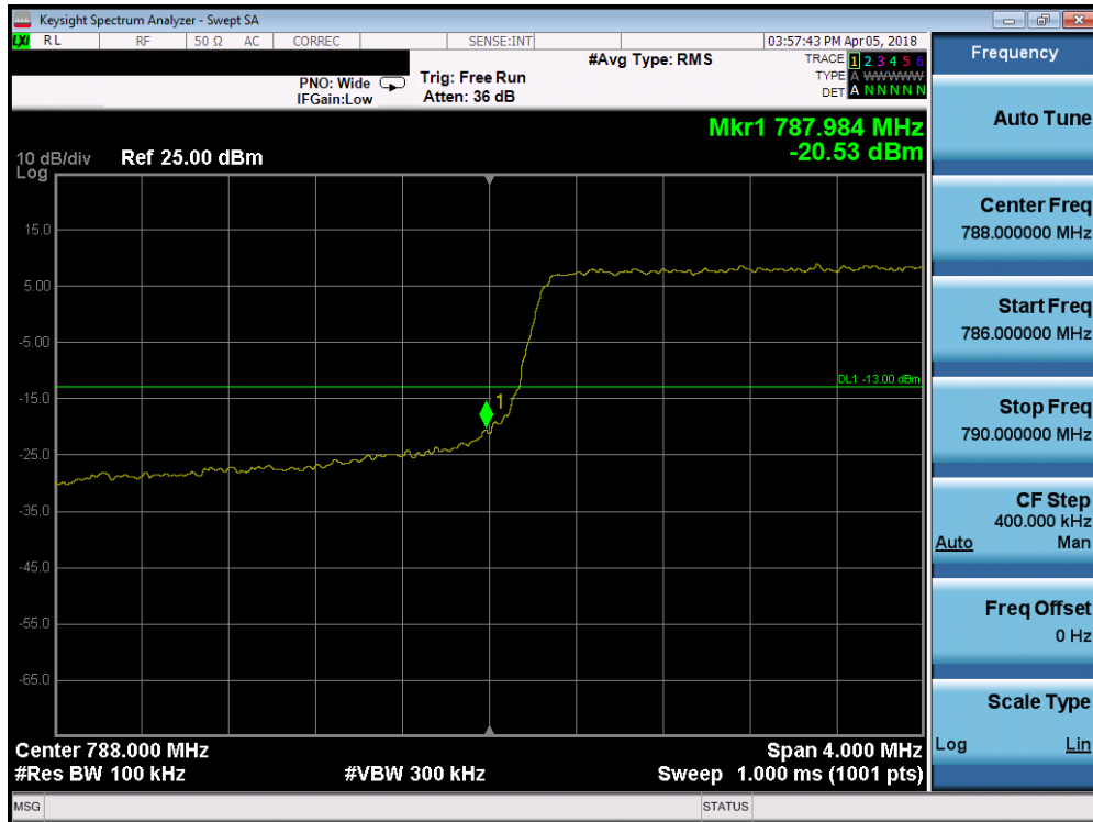
Plot 7-8. Lower Band Edge Plot (Band 14 - 5.0MHz QPSK - Full RB Configuration)
