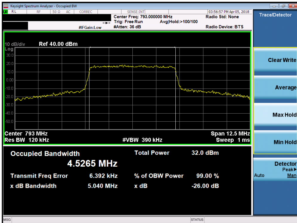
Plot 7-2. Occupied Bandwidth Plot (Band 14 - 5.0MHz 16-QAM - Full RB Configuration)
