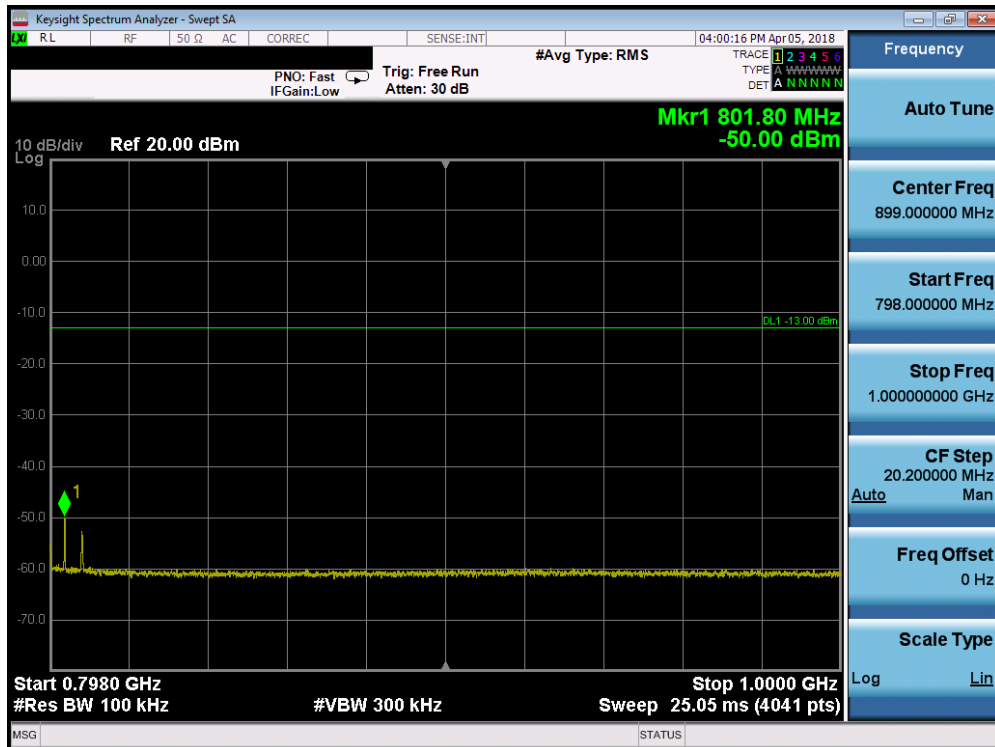
Plot 7-6. Conducted Spurious Plot (Band 14 - 10.0MHz QPSK - RB Size 1, RB Offset 0 - Mid Channel)
