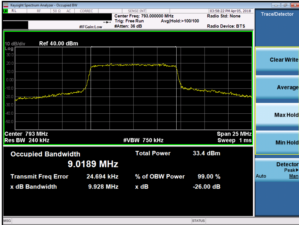
Plot 7-3. Occupied Bandwidth Plot (Band 14 - 10.0MHz QPSK - Full RB Configuration)
