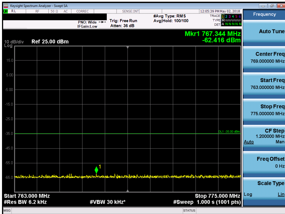
Plot 7-9. Lower Emission Mask Band Edge Plot (Band 14 - 5.0MHz QPSK - Full RB Configuration)
