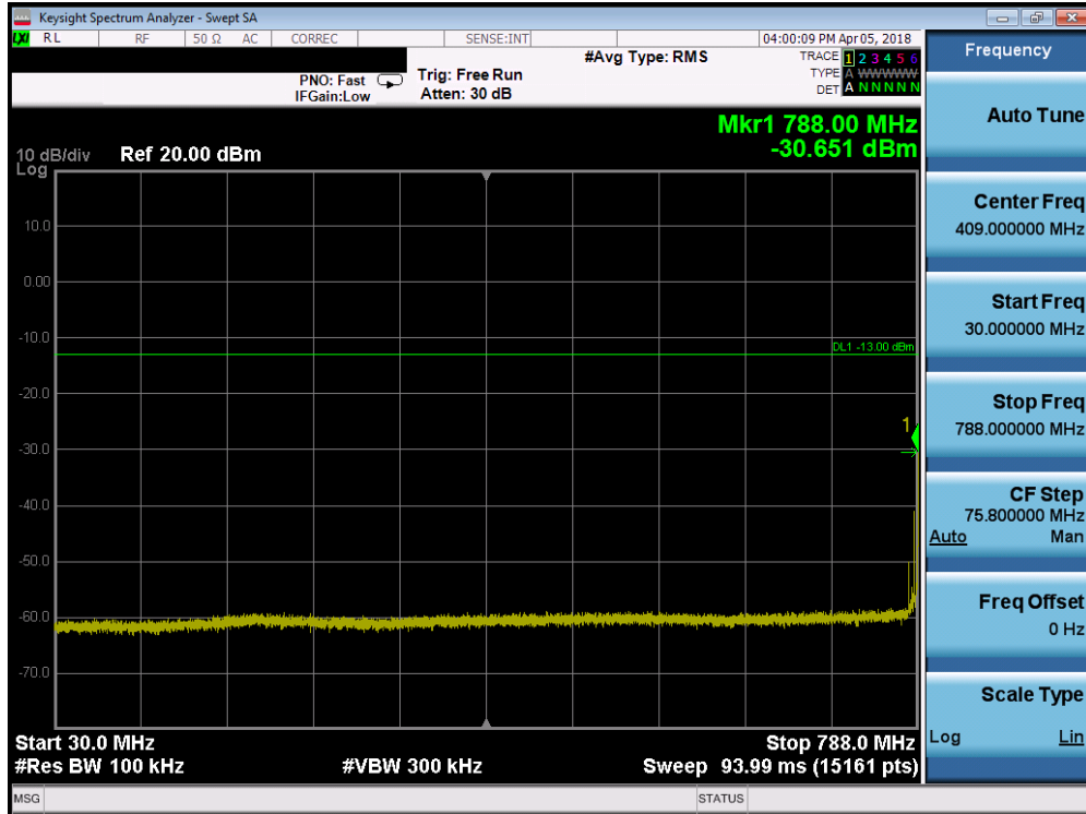
Plot 7-5. Conducted Spurious Plot (Band 14 - 10.0MHz QPSK - RB Size 1, RB Offset 0 - Mid Channel)
