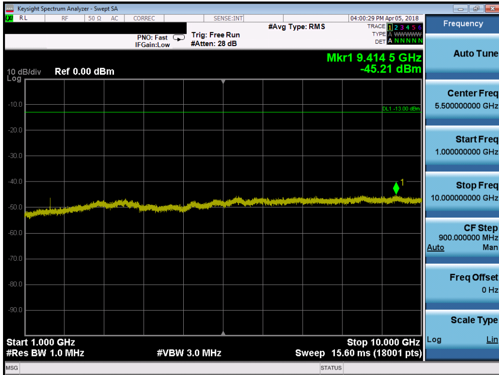
Plot 7-7. Conducted Spurious Plot (Band 14 - 10.0MHz QPSK - RB Size 1, RB Offset 0 - Mid Channel)
