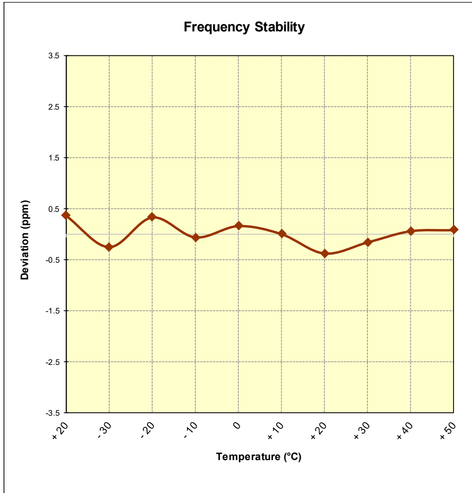
Figure 7-6. Frequency Stability Graph (Band 14)
