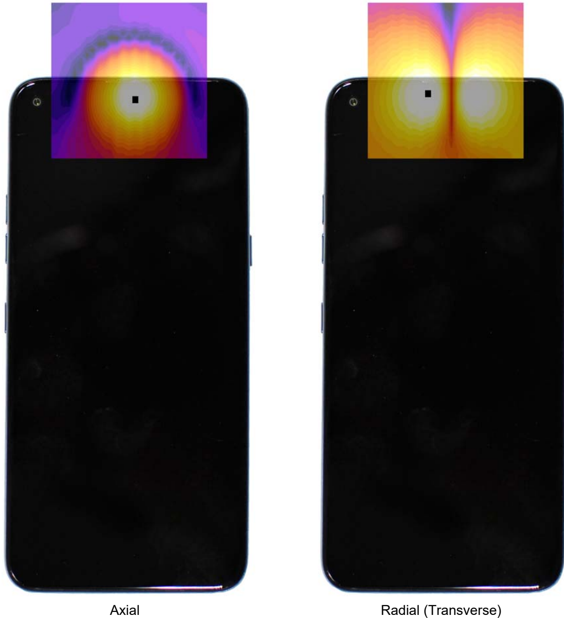
Figure 16-3 T-Coil Scan Overlay Magnetic Field Distributions
